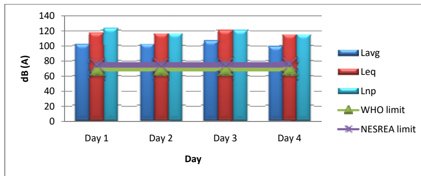
Figure 7: Computed Lavg, Leq and Lnp in comparison with NESREA/WHO Limit
