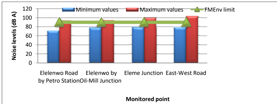
Figure 5: Minimum and maximum Noise levels on Day 4 in comparison with FMEnv limit
