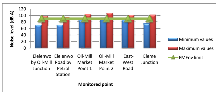
Figure 4: Minimum and maximum Noise levels on Day 3 in comparison with FMEnv limit
