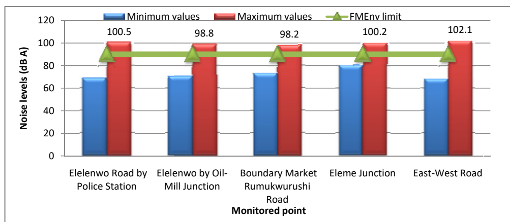
Figure 3: Minimum and maximum Noise levels on Day 2 in comparison with FMEnv limit
