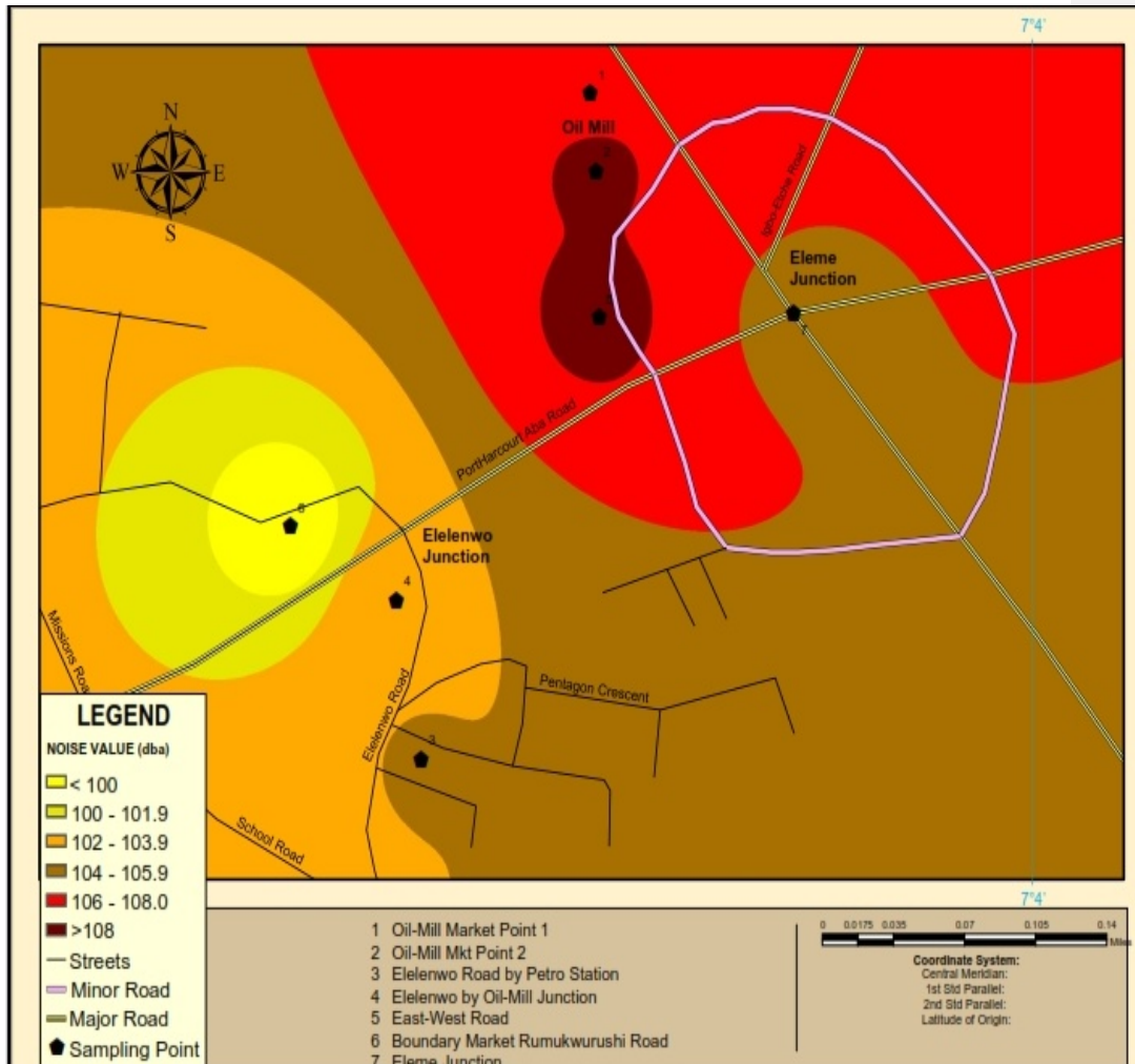
Figure 11: Modelshowing Noise mapping of the Oil Mill Market
