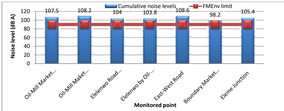
Figure 6: Cumulative Noise levels in comparison with FMEnv limit
