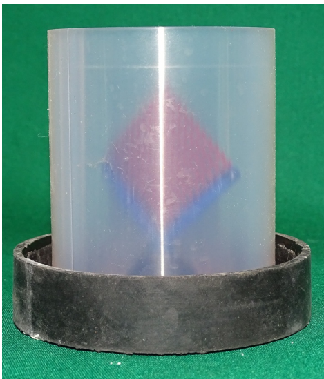
232 Figure 5: Ringless casting technique.
