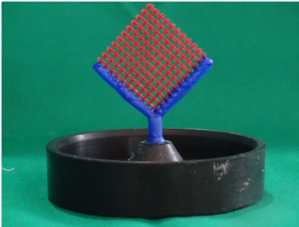
230 Figure 4: Wax mesh pattern attached to crucible former.
