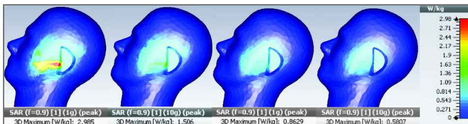
Fig. 6. SAR distribution over SAM phantom human head model with dipole antenna
