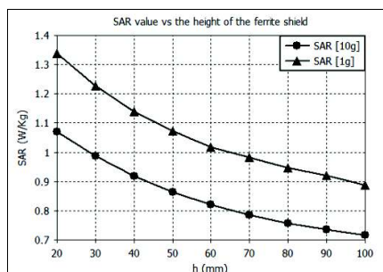
Fig. 14.a. SAR value versus ferrite shield height
