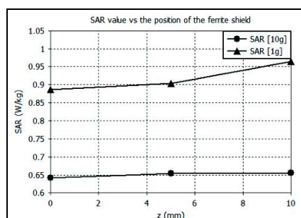
Fig. 5.d. SAR value versus shield position along positive z-axis
