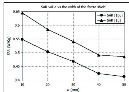
Fig. 10.b. SAR value versus ferrite shield width
