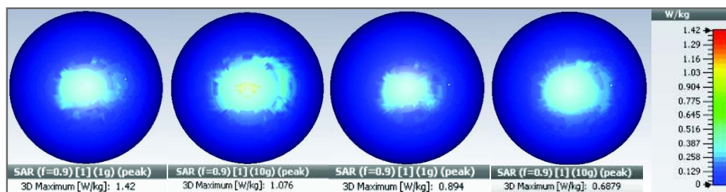
Fig. 17. SAR distribution over two-tissue human head model with helix antenna
