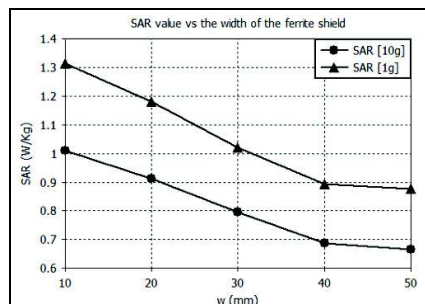
Fig. 18.b. SAR value versus ferrite shield width
