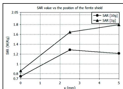
Fig. 7.d. SAR value versus shield position along positive x-axis
