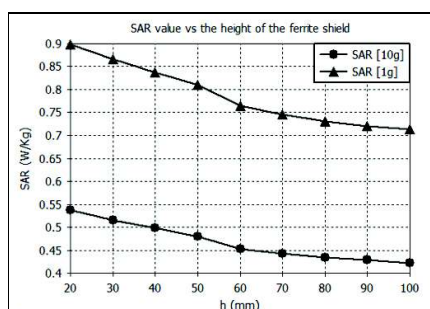
Fig. 3.a. SAR value versus ferrite shield height
