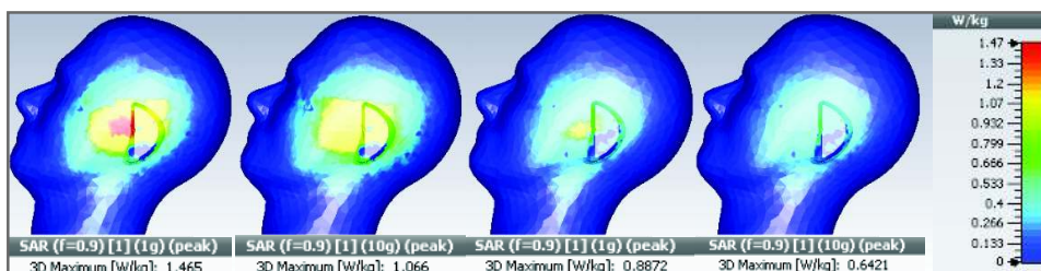
Fig. 4. SAR distribution over SAM phantom human head model with helix antenna
