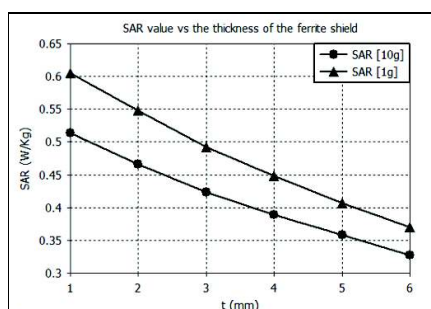
Fig. 10.c. SAR value versus ferrite shield thickness
