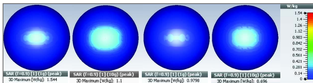
Fig. 19. SAR distribution over two-tissue human head model with dipole antenna
