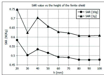
Fig. 16.a. SAR value versus ferrite shield height
