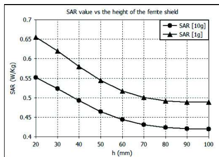
Fig. 10.a. SAR value versus ferrite shield height
