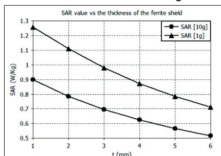
Fig. 20.c. SAR value versus ferrite shield thickness
