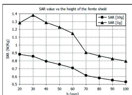
Fig. 7.a. SAR value versus ferrite shield height
