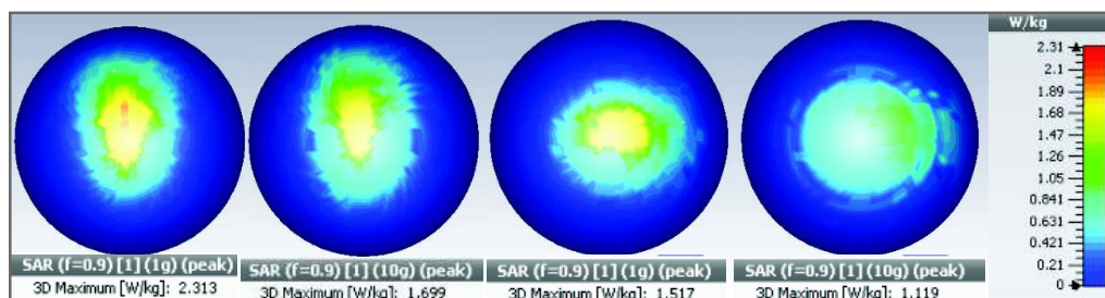
Fig. 11. SAR distribution over six-layer human head model with helix antenna
