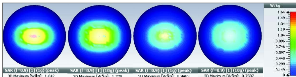
Fig. 13. SAR distribution over six-layer human head model with dipole antenna
