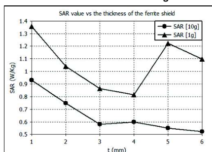
Fig. 7.c. SAR value versus ferrite shield thickness
