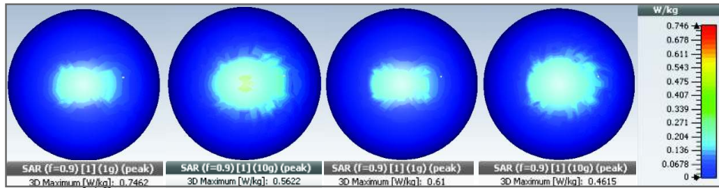
Fig. 15. SAR distribution over two-tissue human head model with monopole antenna The SAR values are swept over the different dimensions of the shield (height, width, thickness and position) as described before in section 4.1.1 and the obtained results are shown in Figs. 16.a-16.d.
