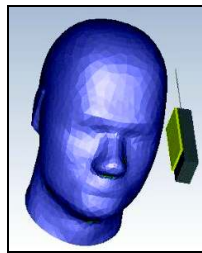
Fig. 1. Complete model used for simulation including SAM phantom model, cell phone, monopole antenna and ferrite shield
