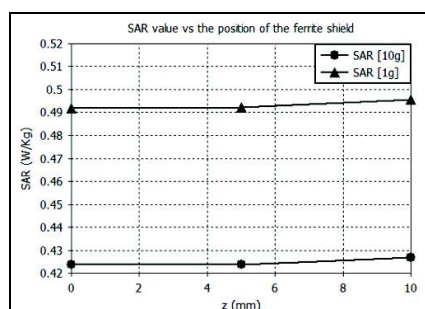
Fig. 10.d. SAR value versus shield position along positive z-axis
