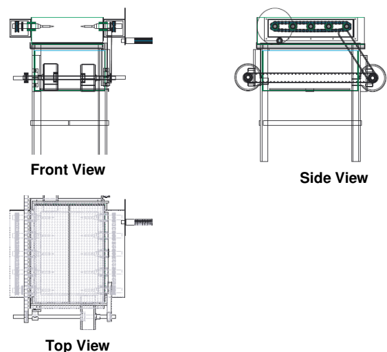
Figure 3. Orthographic View of the Multi-Purpose Roasting Machine
