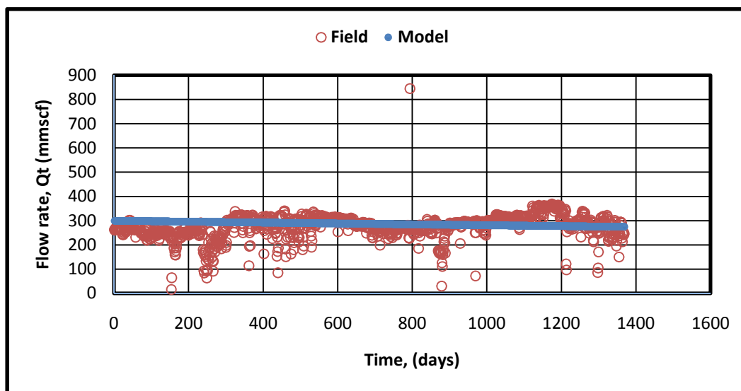
Figure 1: Gas Production Rate - Time Plot (Exponential Model)
