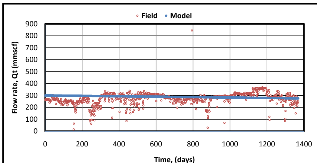
Figure 9: Flow rate - Time Plot (Quadratic Model)
