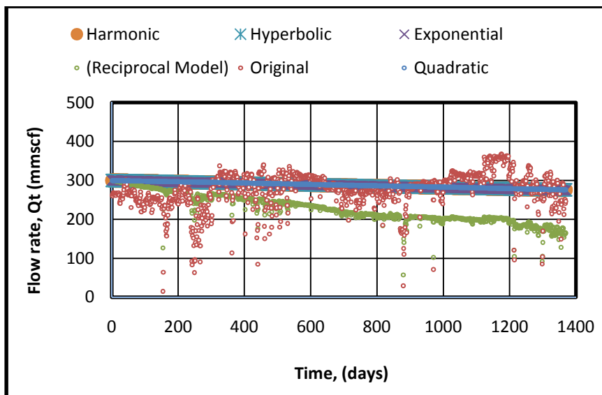
Figure A-7: Gas Production Rate - Time Plot (All Models)
