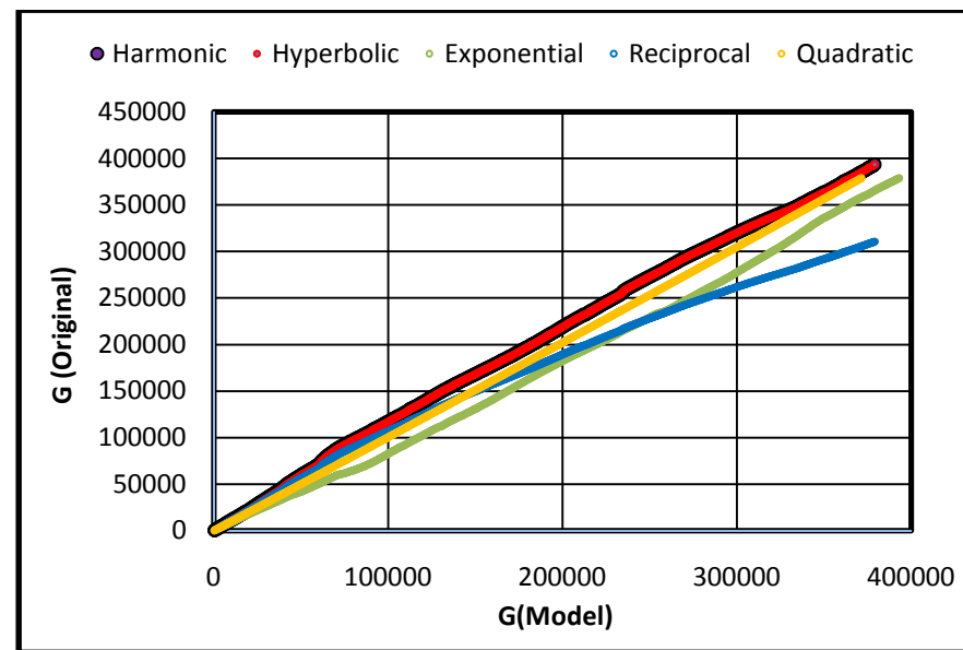
Figure A-8: Field Data – Model Predicted Cumulative Production Plot (All Models)
