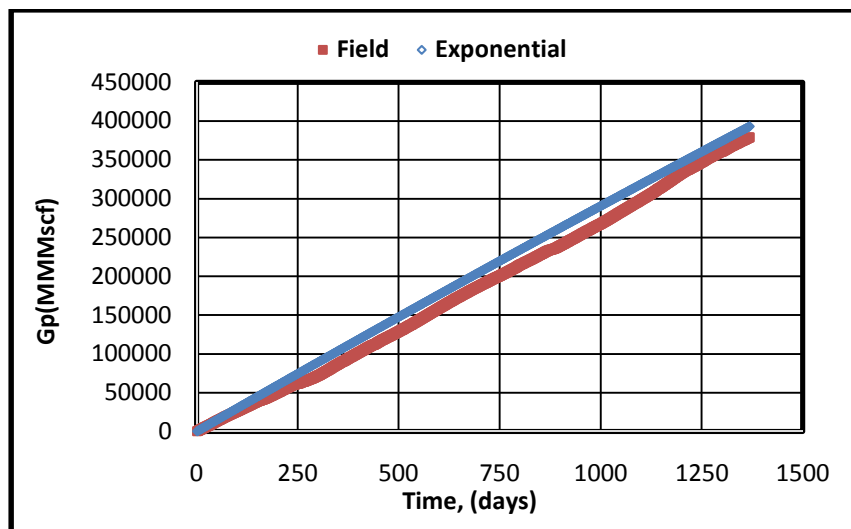
Figure A-1: Cumulative Production - Time Plot (Exponential Model)
