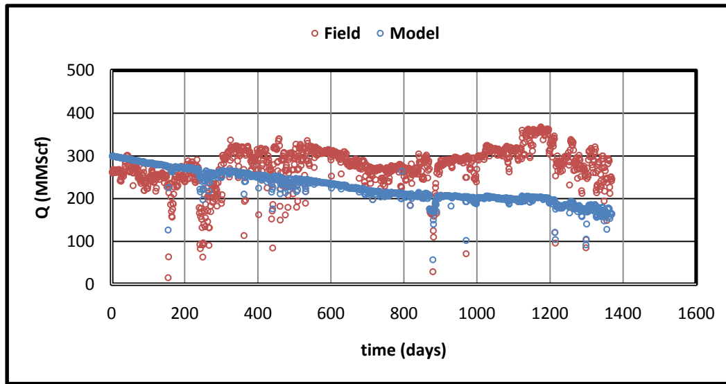
Figure 7: Gas Production Rate - Time Plot (Reciprocal Model)
