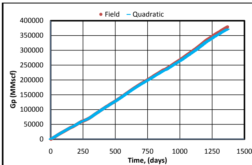
Figure A-5: Cumulative Production - Time Plot (Quadratic Model)
