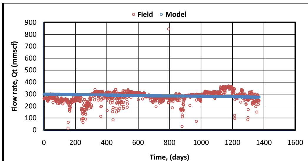
Figure 5: Gas Production Rate - Time Plot (Hyperbolic Model)
