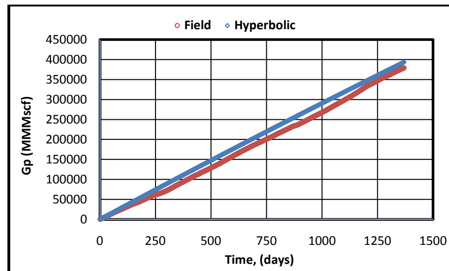
Figure A-3: Cumulative Production - Time Plot (Hyperbolic Model)
