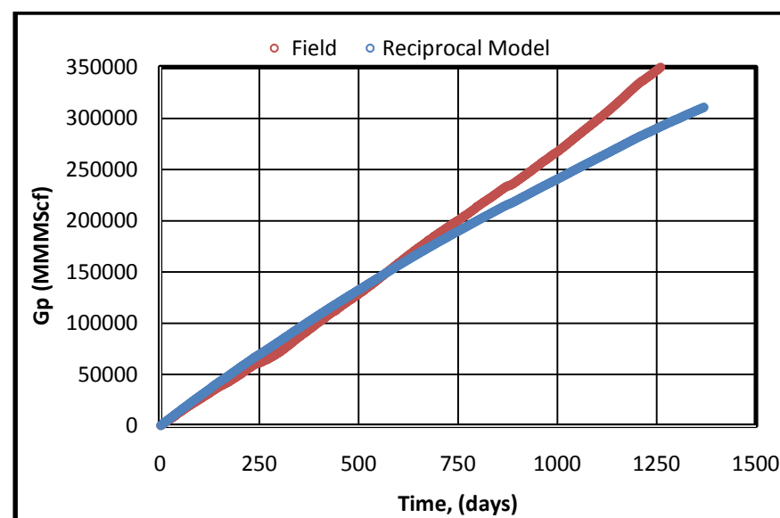
Figure A-4: Cumulative Production - Time Plot (Reciprocal Model)
