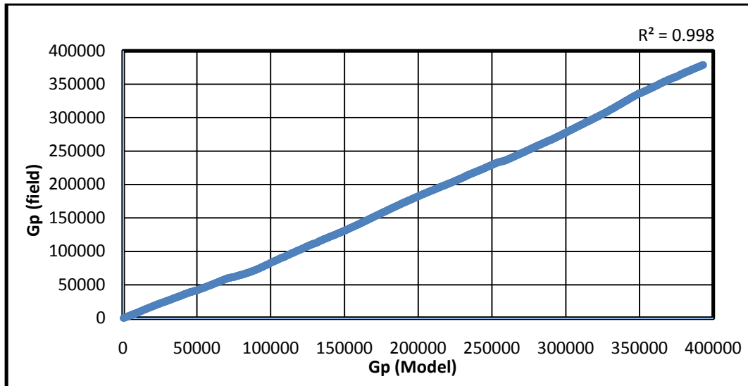
Figure 2: Field Data – Model Predicted Cumulative Production Plot (Exponential Model)
