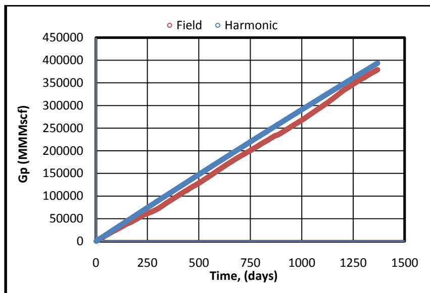
Figure A-2: Cumulative Production vs Time Plot (Harmonic Model)
