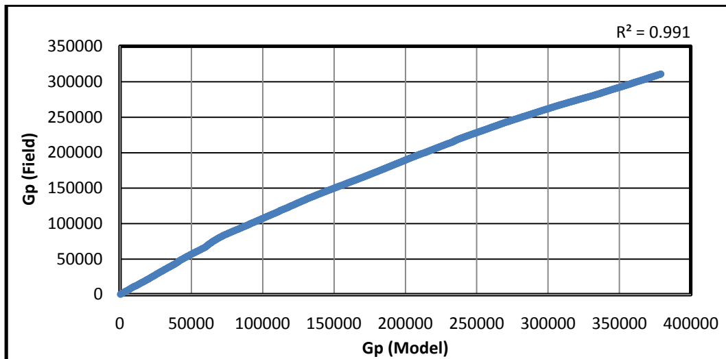
Figure 8: Field Data – Model Predicted Cumulative Production Plot (Reciprocal Model)
