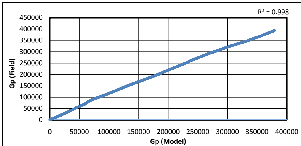
Figure 4: Field Data – Model Predicted Cumulative Production Plot (Harmonic Model)
