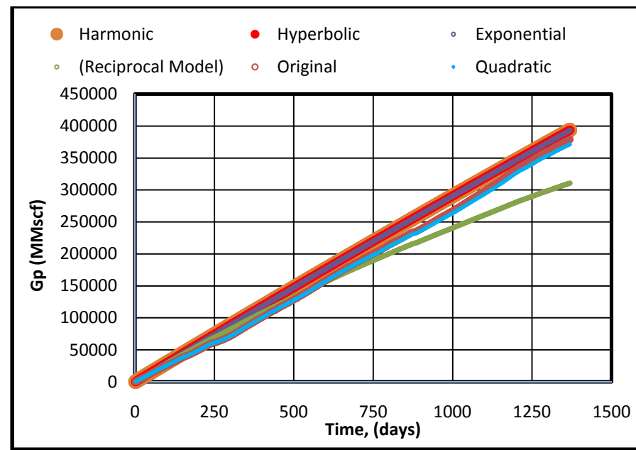
Figure A-6: Cumulative Production - Time Plot (All Models)
