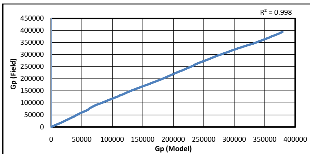
Figure 6: Field Data – Model Predicted Cumulative Production Plot (Hyperbolic Model)
