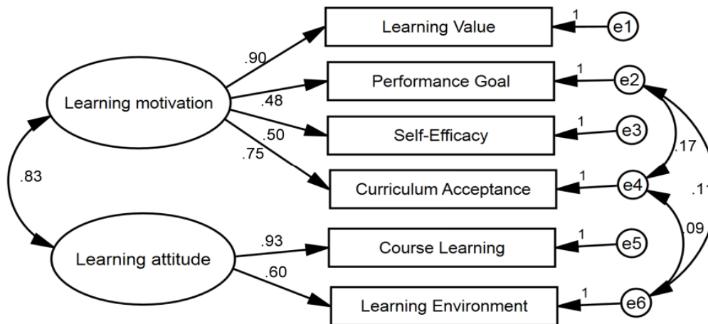
Figure 2: Confirmatory Factor Analysis Model Schematic
