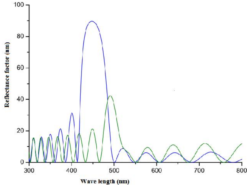
Figure.5.reflectance spectrum calculated according to the parameters of the multilayer observed on the elytron of NecrobiaRufipes . The blue curve corresponds to the dry structure, the green curve in the impregnated water structure. The spectrums were simulated under of incidence of 15^\circ .
