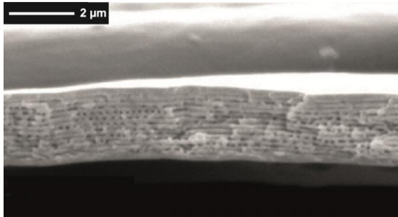
Figure.3. SEM image showing the multilayer the origin of blue reflections of the elytron of NecrobiaRufipes .
