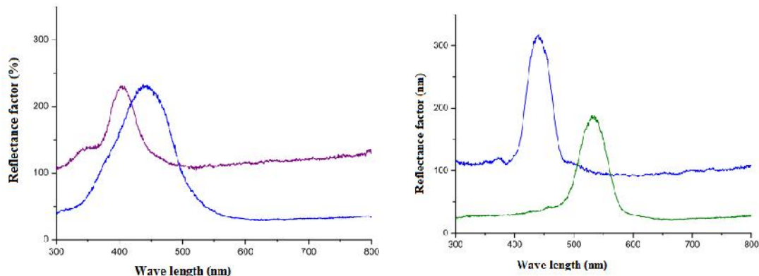
Figure.2. reflectance spectrum of elytron NecrobiaRufipes , left side is the dry structure, the right side structure is impregnated with water, measured for the angles of incidence of 15^\circ and 60^\circ
