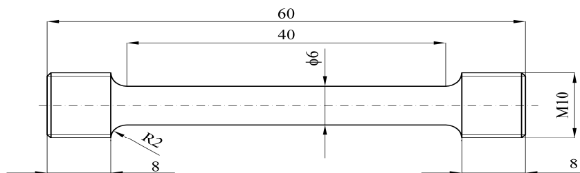
Fig. 2. Specimen for determining of tensile properties of PM and WM [5]
