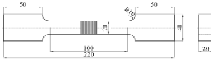
Fig. 1. Specimen for determining of tensile properties of a butt welded joint [4]
