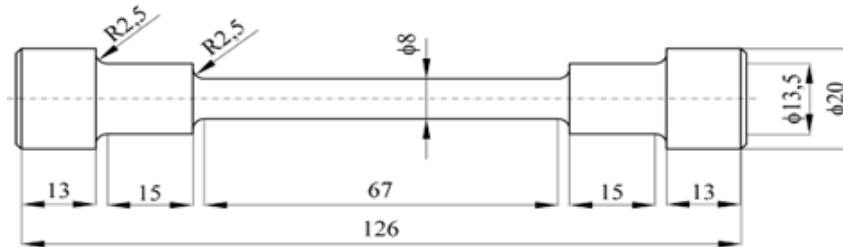
Fig. 4. Specimen for dynamic tests according to ASTM E466 [8]
