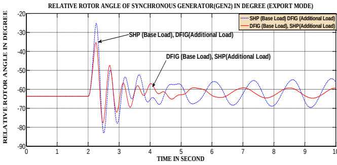
Fig 8: Rotor angle of GEN 2 indicating Load supply by SHP and DFIG and vice versa
