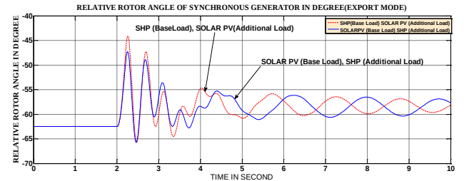
Fig 6: Rotor angle of (GEN2) indicating Load supply by SOLAR PV and SHP and vice versa
