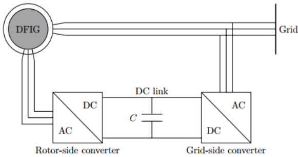
Fig 3: DFIG with its converter [21]
