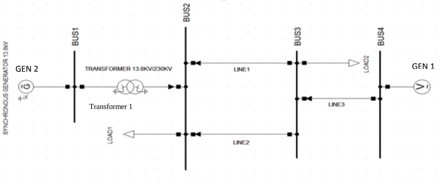
Fig 5: ARRANGEMENT OF THE PROPOSED CONFIGURATION IN DigSILENT
