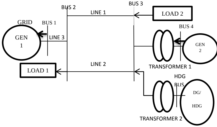
Fig 2: Proposed Modeling Configuration for Export Mode
