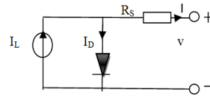
Fig 4: Model for single solar cell
