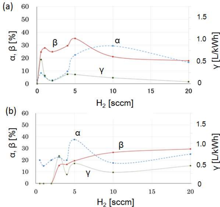
269 Fig. 7. Variations of \alpha , \beta , and \gamma as a function of hydrogen flow rate for (a) separated 270 and (b) mixed gas feedings. Applied voltage is 1.25 kV. CO_2 = 1\text{sccm} .
