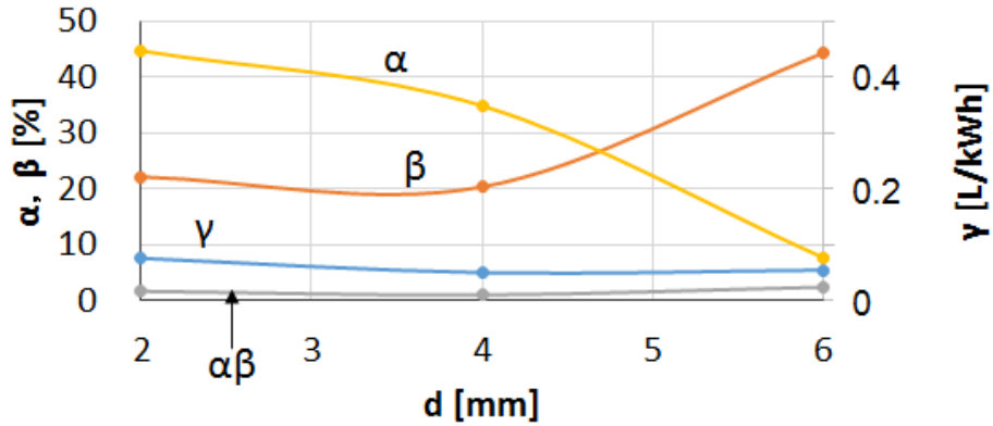
Fig. 3. Variations of \alpha , \beta , \alpha\beta , \gamma as a function of electrode distance d in case of \text{CO}_2/\text{H}_2 = 1\text{sccm}/10\text{ sccm} in a 4-mm-diameter glass tube.
