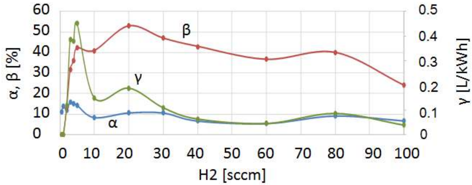
Fig. 4. Variations of \alpha , \beta , and \gamma as a function of H 2 flow rate in case of CO 2 sccm in a 6-mm-diameter glass tube. Electrode distance d = 6 mm.
