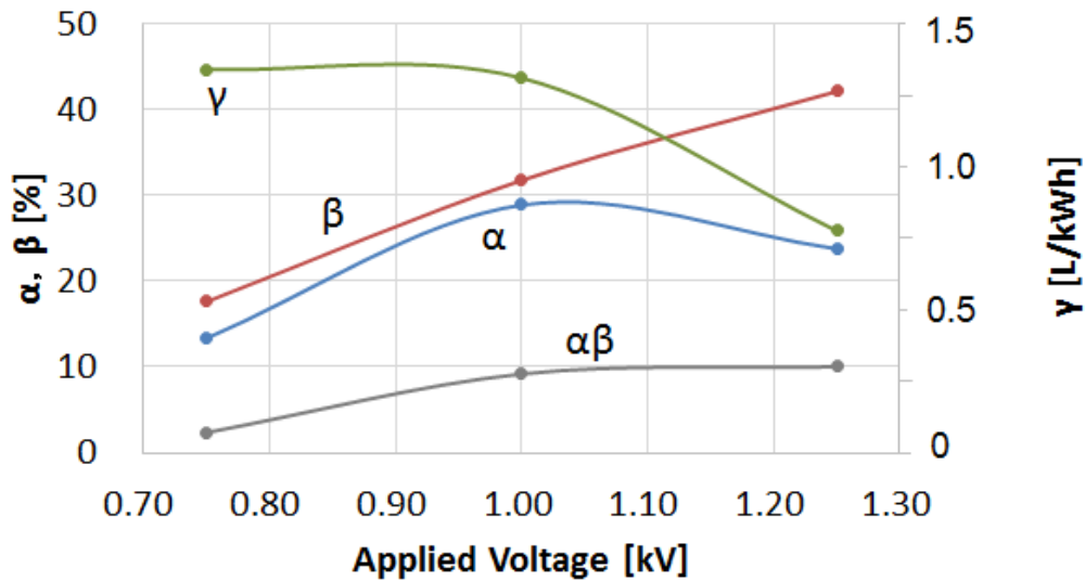
Fig. 5. Variations of \alpha , \beta , \alpha\beta , and \gamma as a function of applied voltage in a 6-mm-diameter glass tube. CO 2 /H 2 = 1sccm/5sccm.
