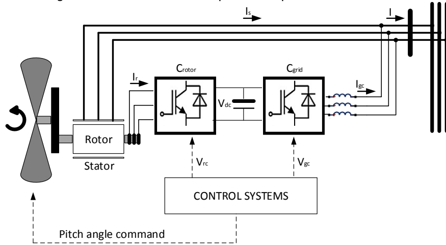
Fig. 1. A simplified DFIG and its connection to the grid
