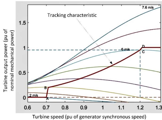
Fig. 2.19. Turbine power characteristics (pitch angle \beta = 0 )
