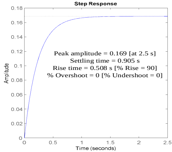
Fig. 2.1. Wind turbine rotor pitch open-loop unit step response
