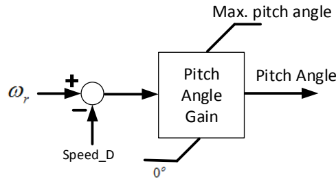
Fig. 2.18. Pitch angle control system
