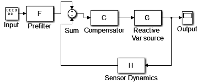
Fig. 2.7. Architecture of reactive power management system
