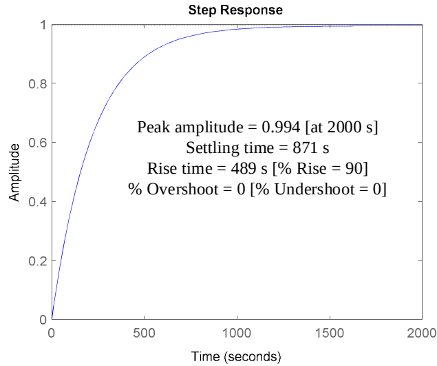
Fig. 2.12. DC bus voltage open-loop unit step response
