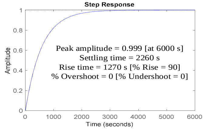
Fig. 2.3. Generator open-loop unit step response
