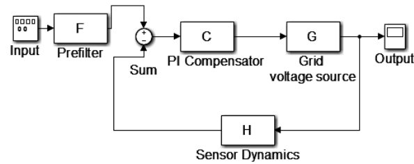
Fig. 2.10. Architecture of grid voltage regulator
