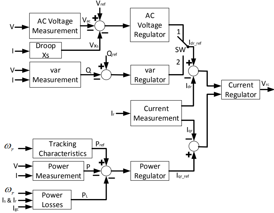
Fig. 2.20. Rotor-side converter voltage and reactive power control systems
