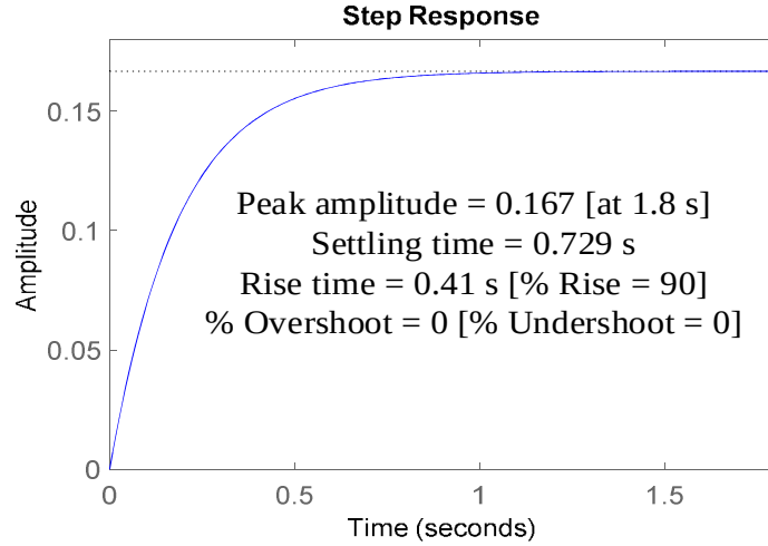
Fig. 2.9. Voltage source open-loop unit step response
