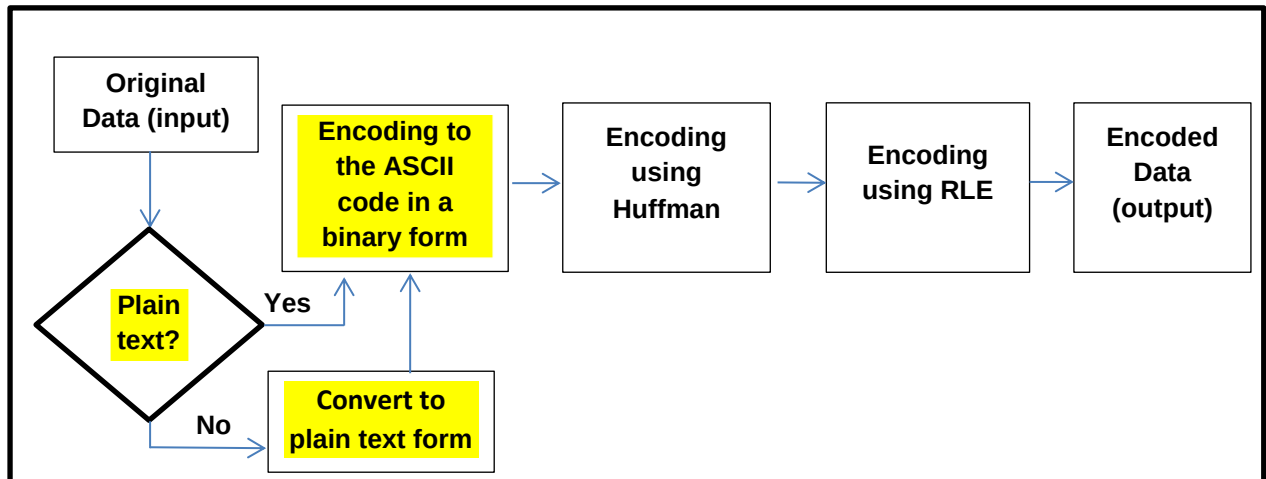
Fig. 1. Process of Encoding using Huffman and RLE techniques
