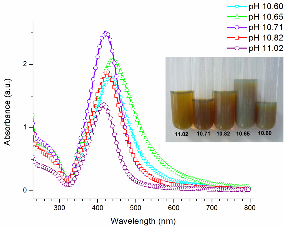
Figure 1. UV-vis spectra of silver nanoparticle solutions obtained at different pH values. The inset shows the typical color of these solutions.
