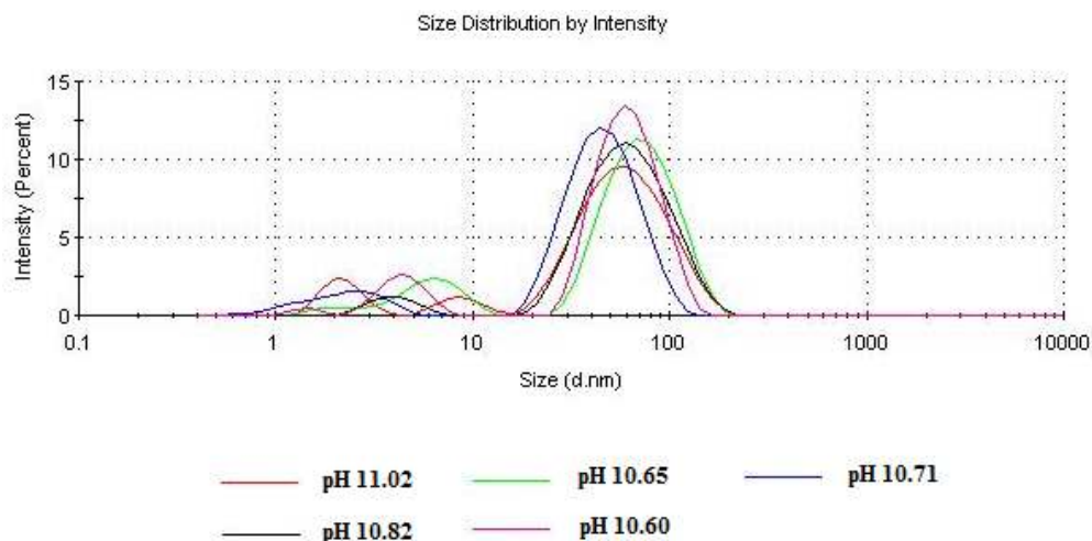
Figure 2. Size distribution of silver nanoparticles synthesized at different pH values.
