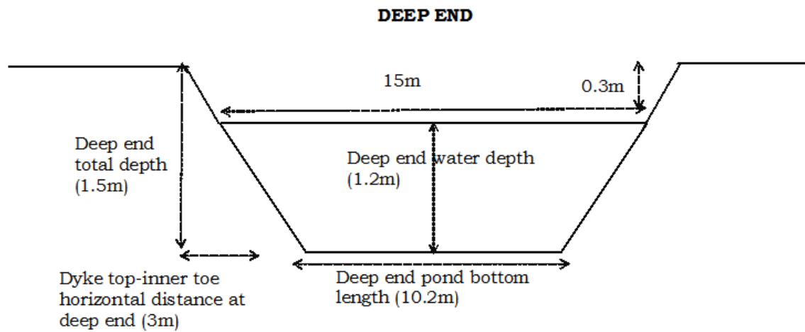
376 Figure 5: Width wise section of the pond at the deep end showing the various measurements
