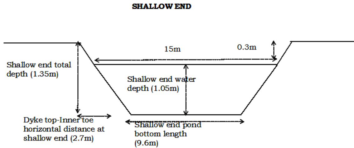
370 Figure 4: Width wise section of the pond at the shallow end showing the various 371 measurements
