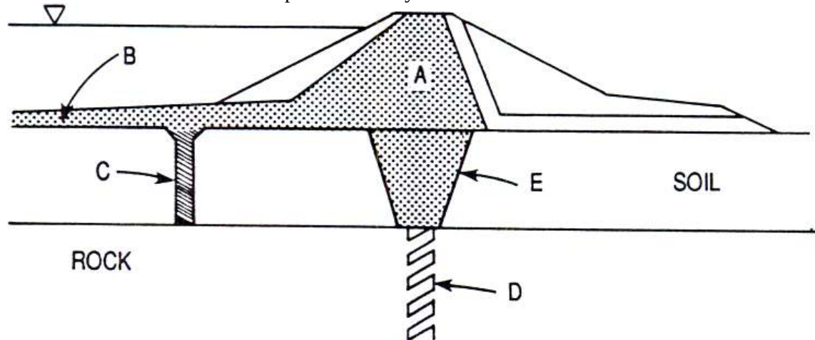
Figure1: Features for reducing seepage through pond and their foundation
