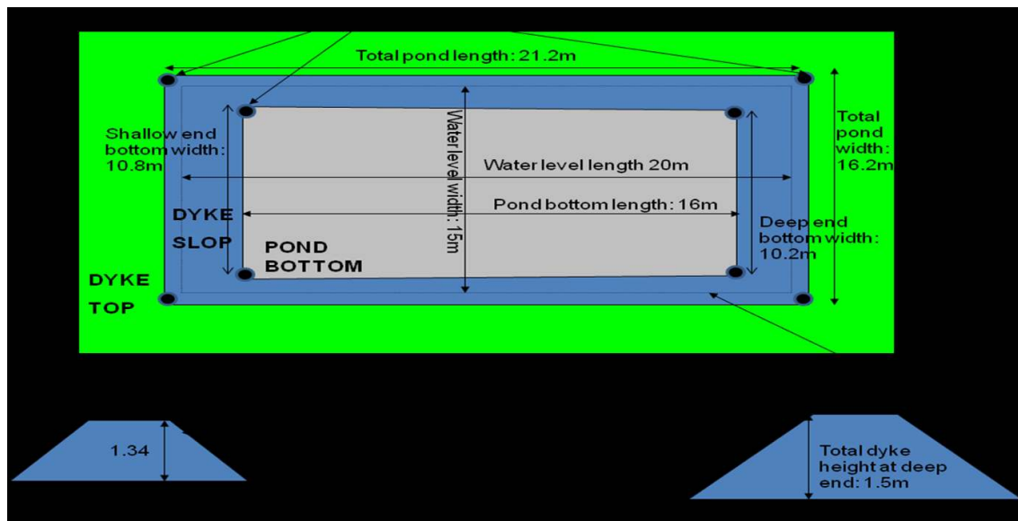
Figure 6: Plan view showing the pegging positions for a 300 m 2 pond
