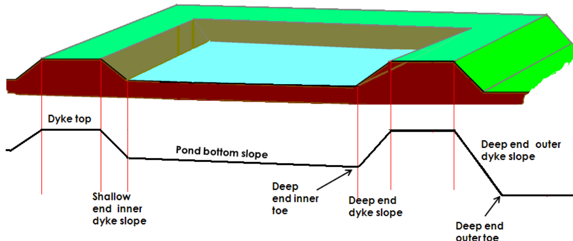
Figure 2: A cross section of an earthen fish pond showing the slopes and the dykes
