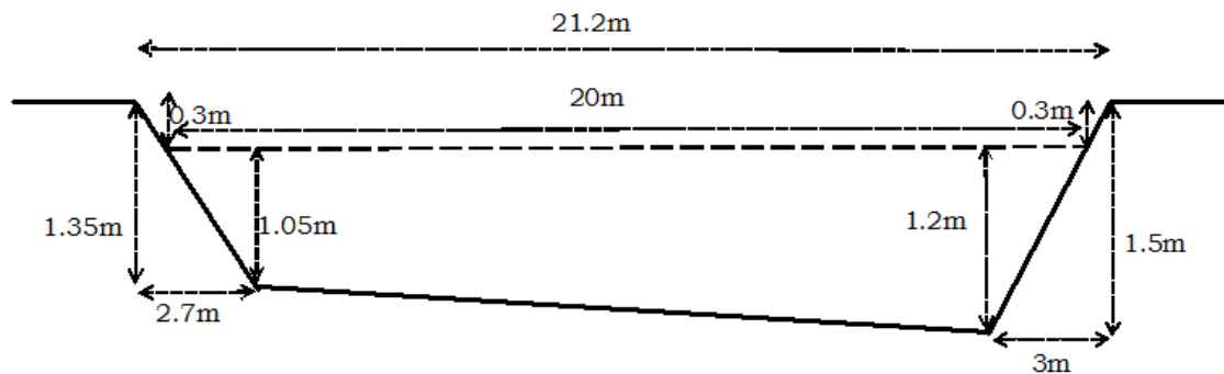
Figure 3: Length wise section of the pond showing the various measurements
