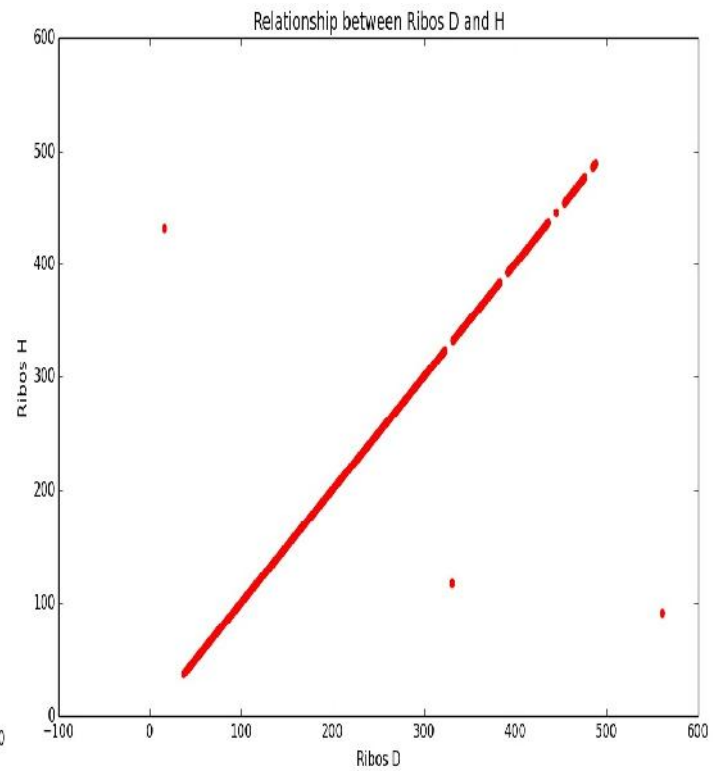
Fig. 4: DNA sequence relations between Ribos D and H isolates
