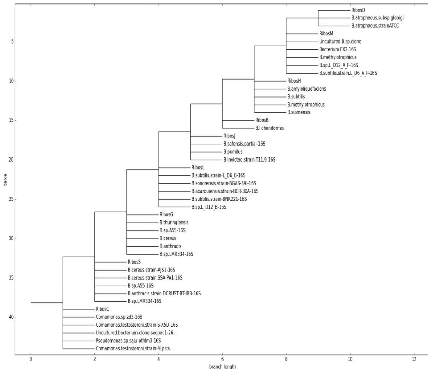
Fig. 10: Phyletic relatedness of isolated Bacillus species and database closely related sequences
