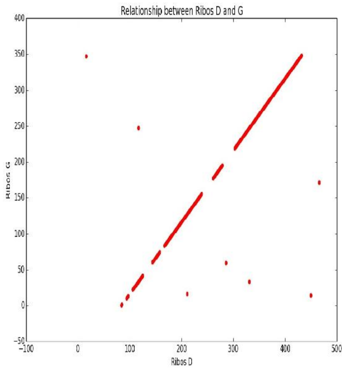
Fig. 3: DNA sequence relations between Ribos D and G isolates
