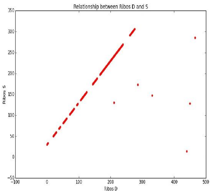
Fig. 8: DNA sequence relations between Ribos D and S isolates
