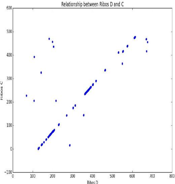
Fig. 2: DNA sequence relations between Ribos D and C isolates
