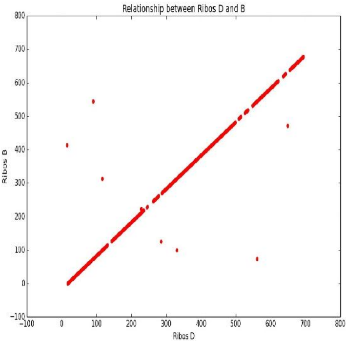
Fig. 1: DNA sequence relations between Ribos D and B isolates
