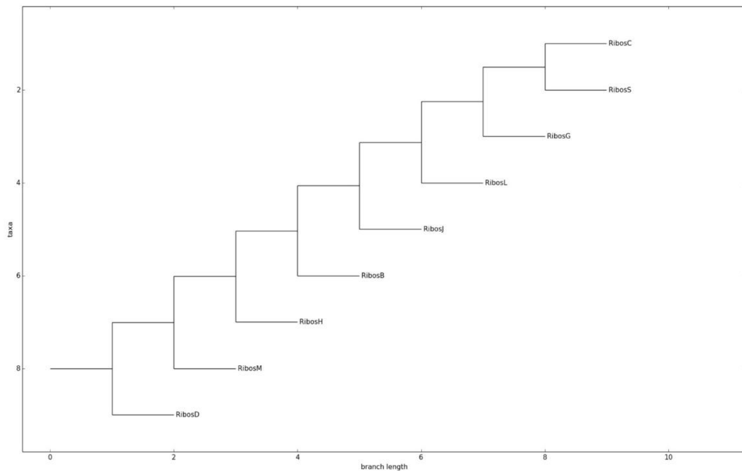
Fig. 9: Genetic relatedness of Bacillus species isolated from ready-to-eat (RTE) foods
