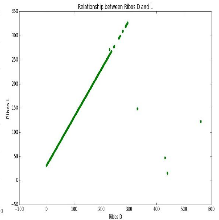
Fig. 6: DNA sequence relations between Ribos D and L isolates
