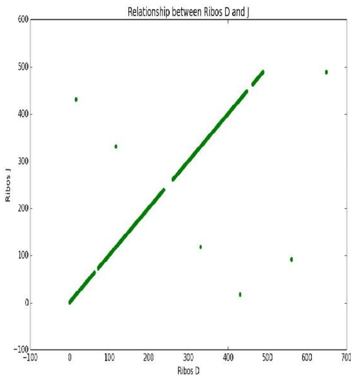
Fig. 5: DNA sequence relations between Ribos D and J isolates
