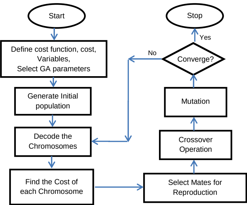
Figure 2: Flowchart of Genetic Algorithm
