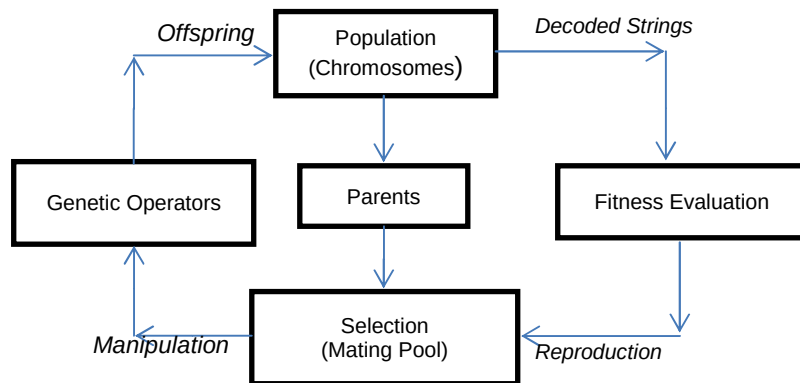
Figure 1: The Generic Algorithm Model
