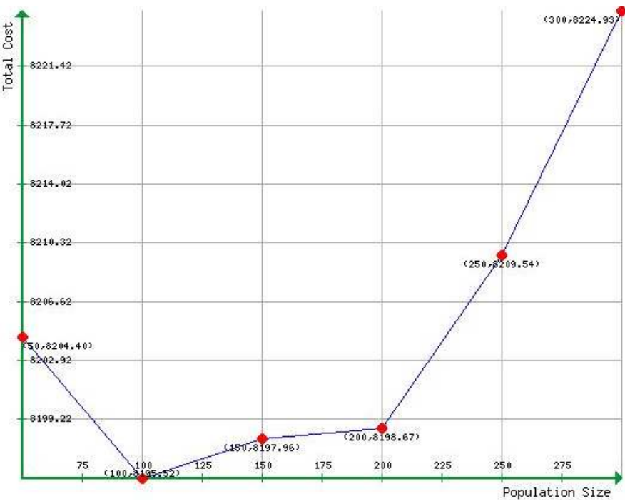
Figure 3: A Graph of Population Size Versus Total cost (Pd = 850MW)
