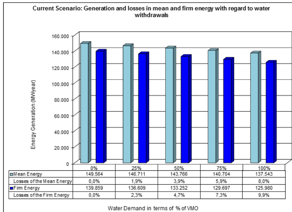
Figure 3: Comparison between average and firm energy generation in the current scenario.
