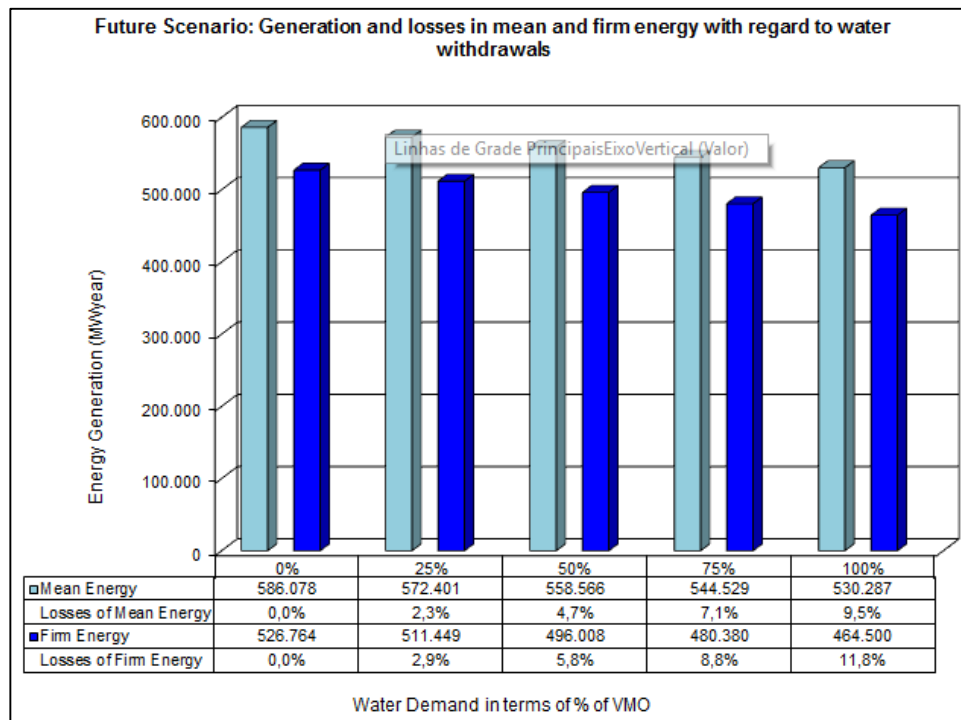
Figure 4: Comparison between average and firm energy generation in the future scenario.
