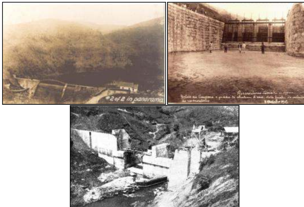
Photos 2 to 4: Construction of dams for the Coronel Fagundes, Piabanha and Morro Grande SHPs, respectively. Source: ME, 2000.
