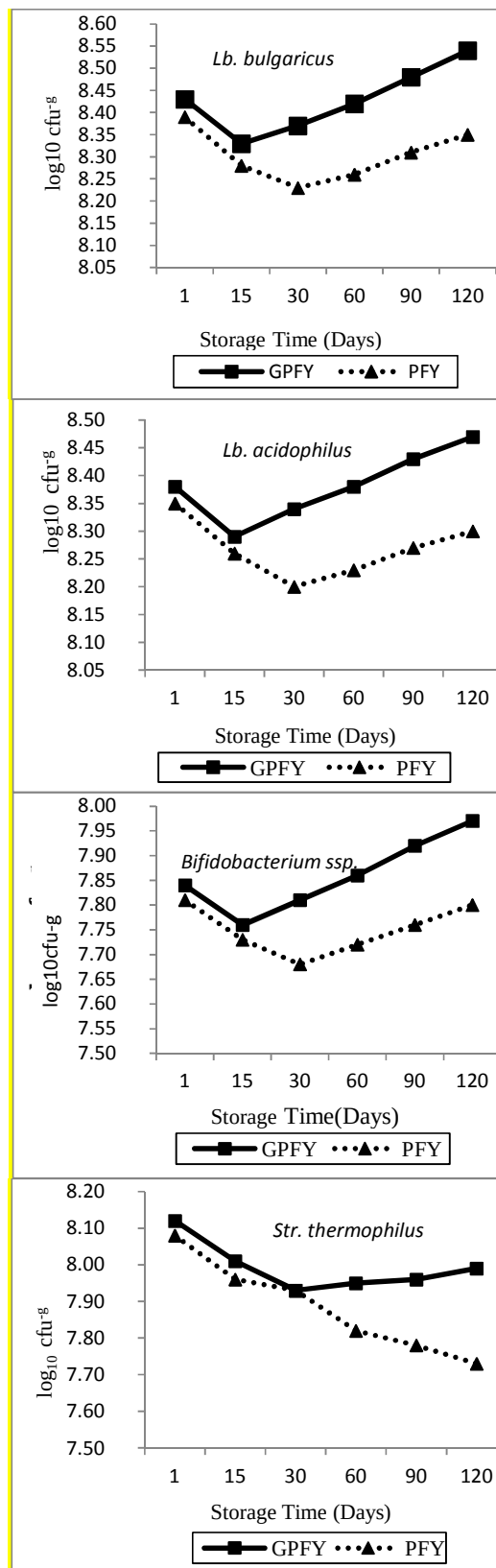
Figure 2. Lb. bulgaricus , Lb. acidophilus , Bifidobacterium ssp. and Str. Thermophilus counts in PY samples during storage
