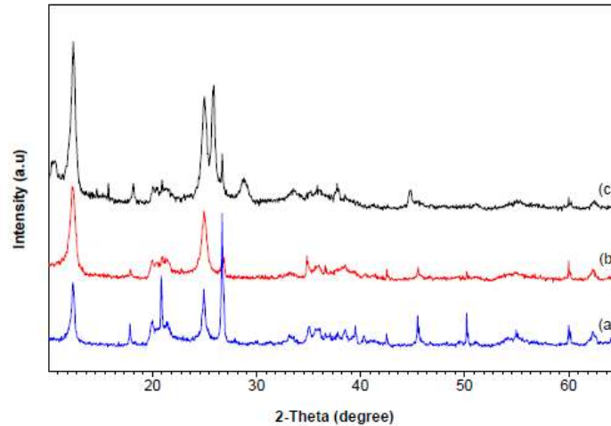
Figure 1: X-Ray diffraction of Ekiti and Osun state (a) Idoka (b) Ilesha (c) Ijero
