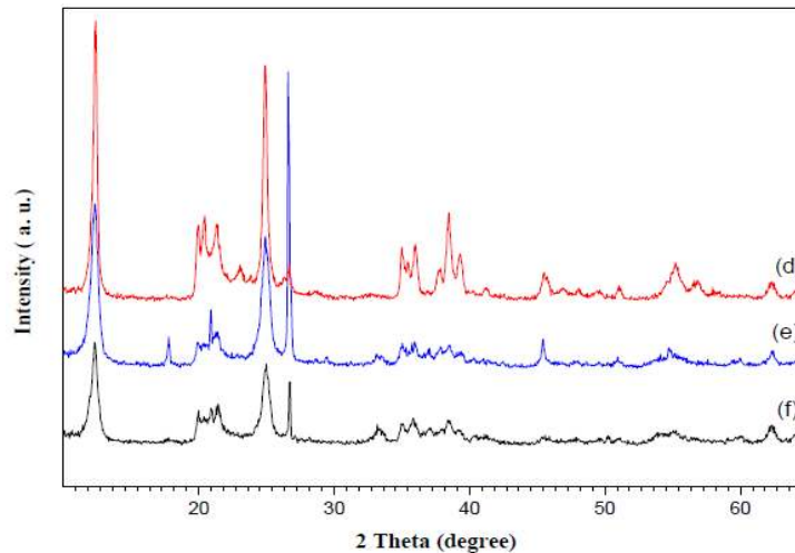
Figure 2: X-Ray diffraction of Ondo state clays (d) Ijapo (e) Barrack (f) Ondo
