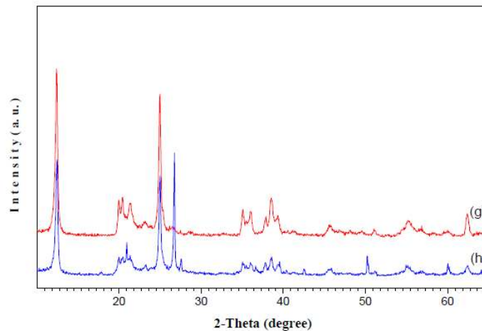
Figure 3: X-Ray diffraction of Ogun and Lagos clay (g) Ajebo (h) Ibafo
