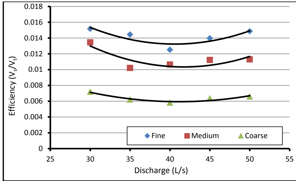
Fig.6. The relation between jet pump sand removal's efficiency ( V_s/V_t ) and discharge for different sand gradations
