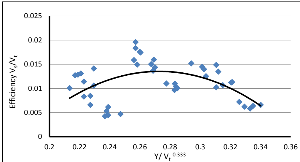
Fig.5. The relation between jet pump sand removal's efficiency ( V_s/V_t ) and ( Y/V_t^{0.33} ) NB: those results are results from the analyzing of the experimental data. ( V_s/V_t ) : jet pump sand removal's efficiency as ( V_s ) : volume of removed soil; ( V_t ) :total volume of jet pump out put (mixture sand / water); ( Y ) is the water depth of the flume.
