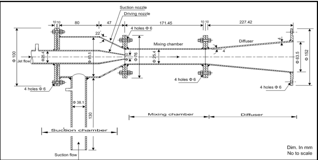
Fig .2. Principal components of the used jet-pump [11]
