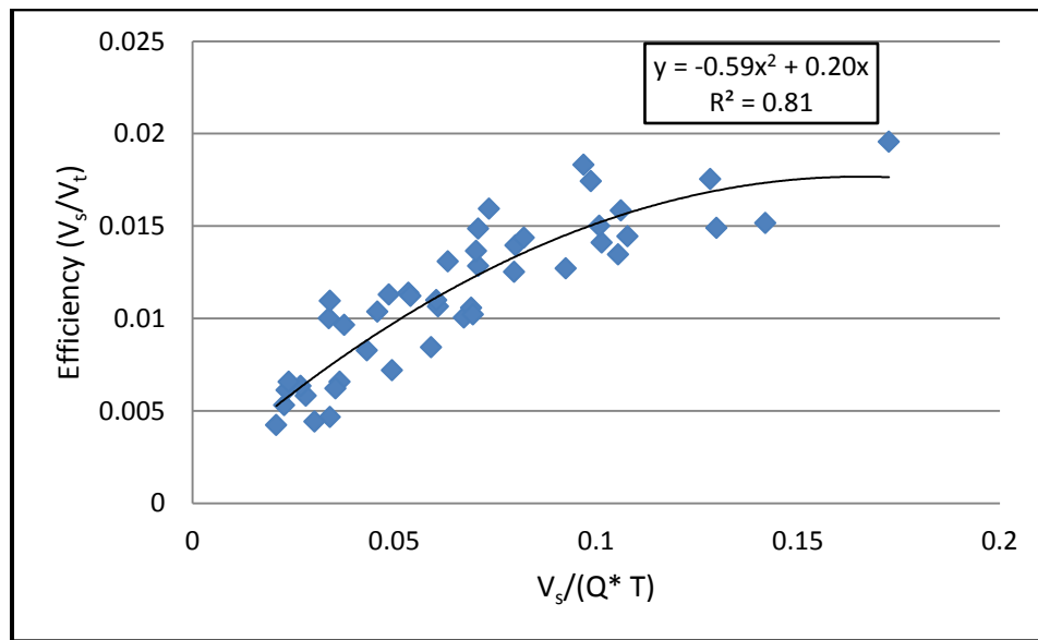
Fig.8. The relation between jet pump sand removal's efficiency ( V_s/V_t ) and ( V_s/QT )
