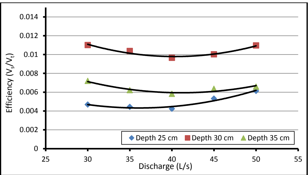
Fig.4. The relation between jet pump sand removal's efficiency ( V_s/V_t ) and discharge for different water depths
