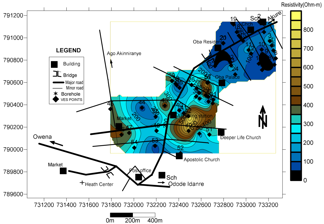
Fig. 5: Contour Map showing the resistivity distribution of the Aquifer Units
