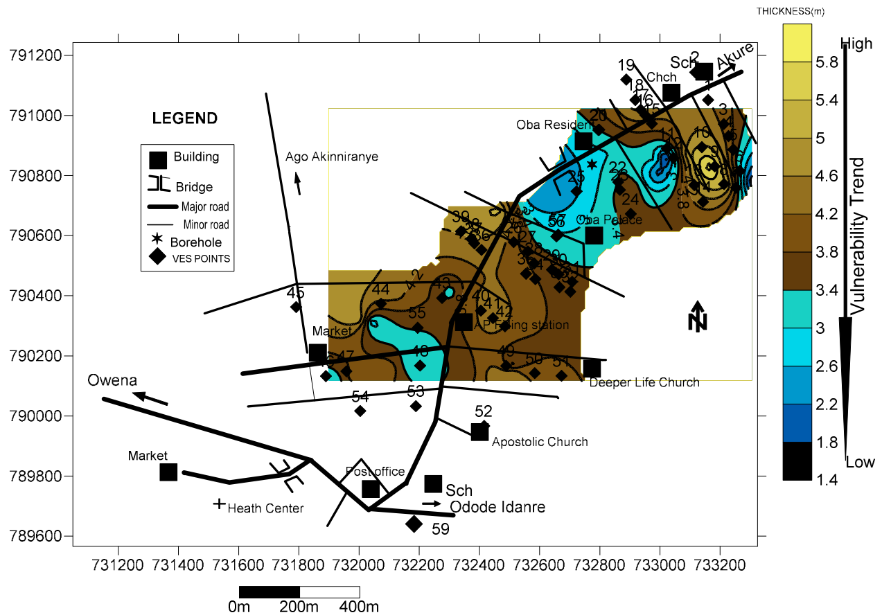
Fig. 4: Thickness Map showing unconsolidated materials overlying the basement at Alade.
