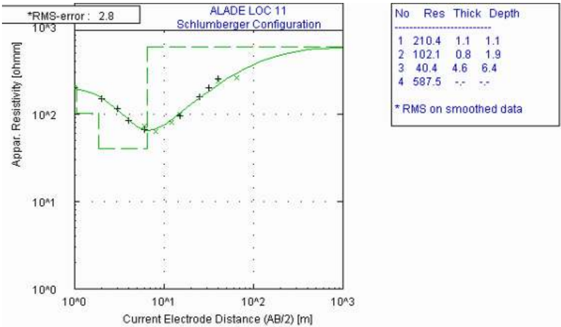
Fig.2: Typical Vertical Electrical Sounding Curves from the Study Area
