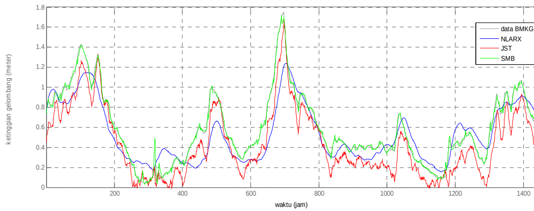
Fig.5. The actual and result of wave height predictors in 1 hour later in A, B, and C using SMB, ANN, NLARX
