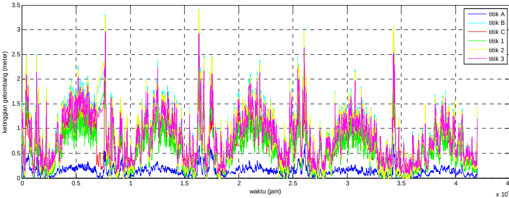
191 192 Fig. 4. The mean of wave height in 6 locations in sea line of Surabaya – Banjarmasin 193
