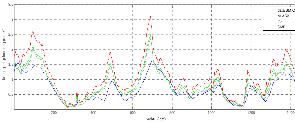
Fig. 6. The actual and the result of wave height predictor in 1 hour later in points 1, 2, and 3 using SMB, ANN, NLARX
