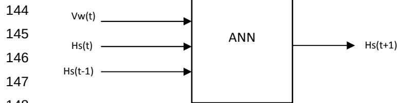
149 Fig. 2 Block diagram of ANN designed predictors
