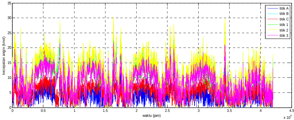
188 189 Fig. 3. The mean of wind speed in 6 locations in sea line of Surabaya – Banjarmasin 190
