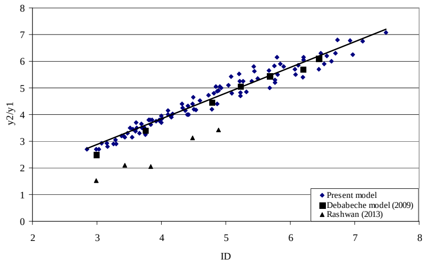
Figure 6 Comparison of model Equation 5 with Debabeche and Rashwan models
