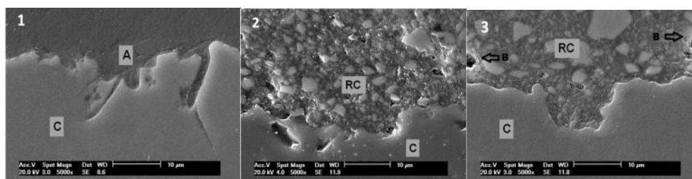
Fig. 1.2 and 3 – SEM images (5000x): (1) - Interface between Scotchbond MultiPurpose adhesive and feldspathic ceramic etched with 10% hydrofluoric acid (5000x): (A) adhesive; (C) ceramic. (2) - Interface between RelyX ARC resin cement and feldspathic ceramic etched with 10% hydrofluoric acid: (RC) resin cement; (C) ceramic. (3) - Interface between RelyX U100 resin cement and feldspathic ceramic etched with 10% hydrofluoric acid: (RC) resin cement; (C) ceramic; (B) voids in cement, see arrows .
