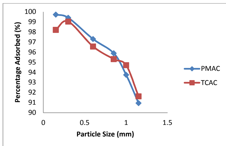
Figure 4. Effect of particle size on Pb(II) adsorption by PMAC and TCAC
