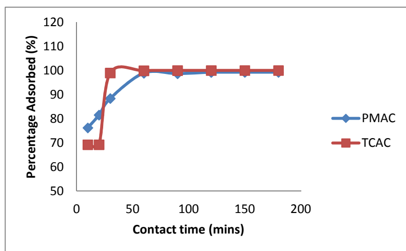
Figure 8. Effect of contact time on Pb(II) adsorption by PMAC and TCAC
