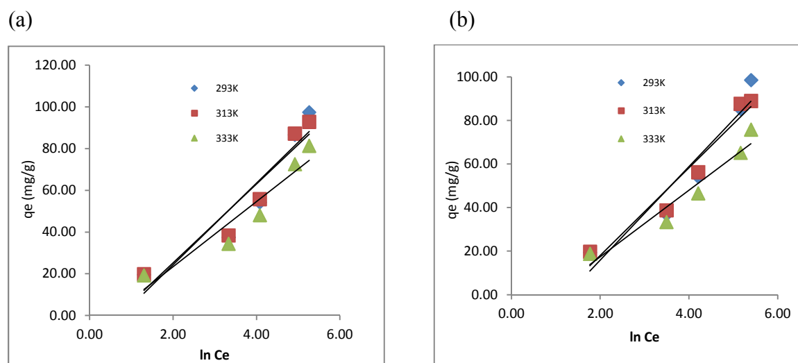
Figure 12. Temkin plot for Pb(II) adsorption onto (a) PMAC, (b) TCAC
