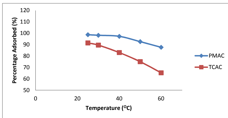
Figure 9. Effect of Temperature on adsorption of Pb(II) by PMAC and TCAC
