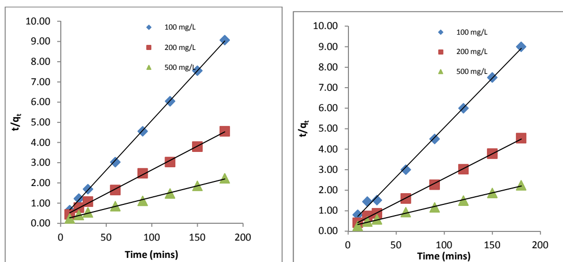
Figure 15. Pseudo-second-order kinetic plot for Pb(II) adsorption on (a) PMAC, (b) TCAC
