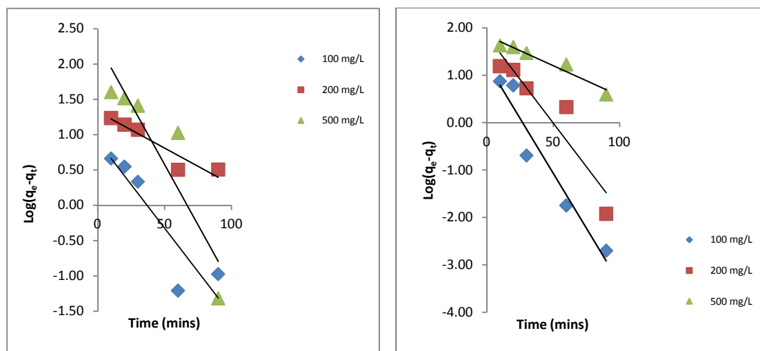
Figure 14. Pseudo-first-order kinetic plot for Pb(II) adsorption on (a) PMAC, (b) TCAC
