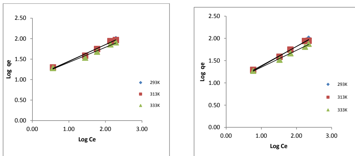
Figure 11. Freundlich plot for Pb(II) adsorption onto (a) PMAC, (b) TCAC
