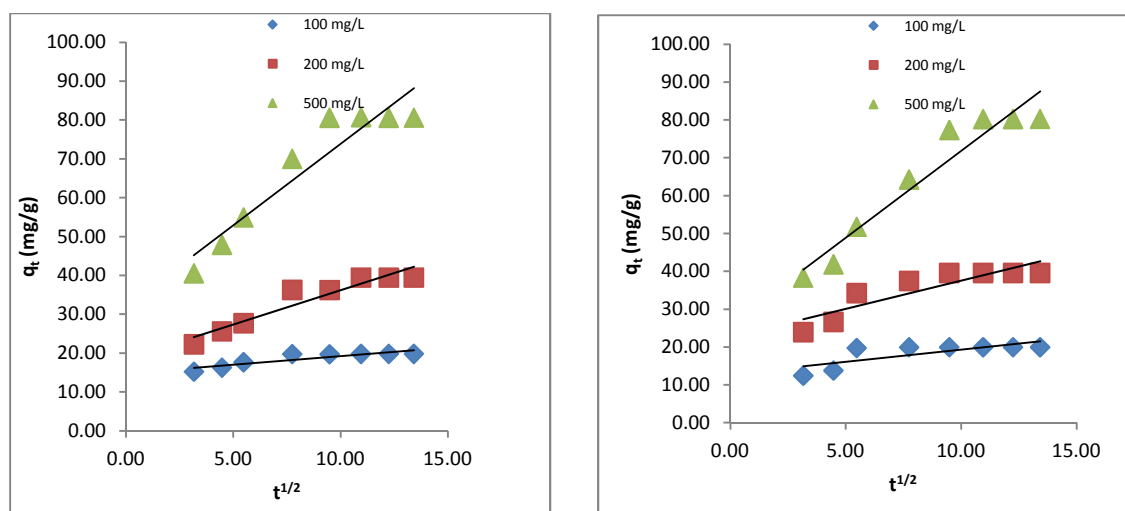
Figure 16. Intraparticle diffusion kinetic plot for Pb(II) adsorption on (a) PMAC, (b) TCAC
