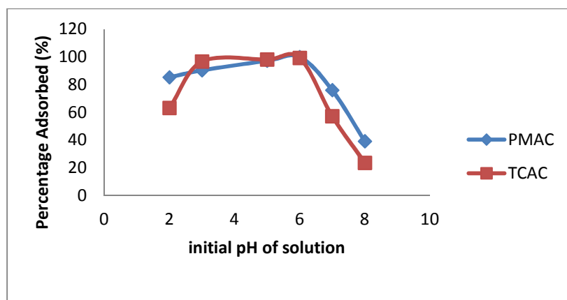
Figure 5. Effect of initial solution pH on Pb(II) adsorption by PMAC and TCAC.
