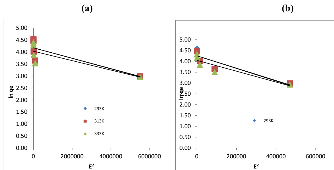
Figure 13. D-R plot for Pb(II) adsorption on (a) PMAC, (b) TCAC
