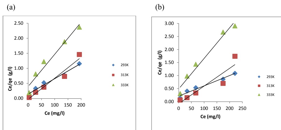
Figure 10. Langmuir plot for Pb(II) adsorption onto (a) PMAC, (b) TCAC
