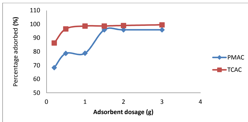
Figure 6. Effect of adsorbent dosages on Pb(II) adsorption on PMAC and TCAC.
