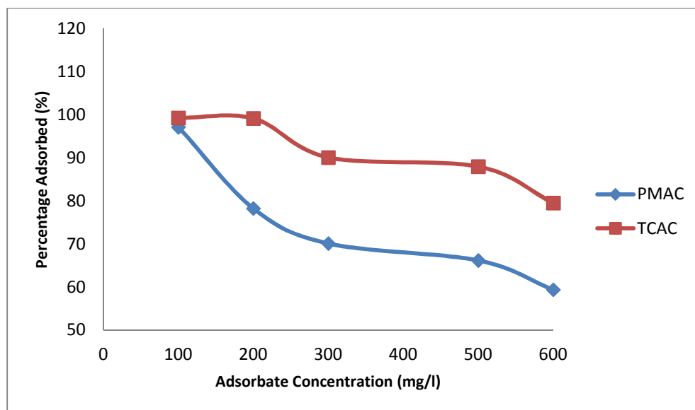
Figure 7. Effect of adsorbate concentration on adsorption of Pb(II) onto PMAC and TCAC.
