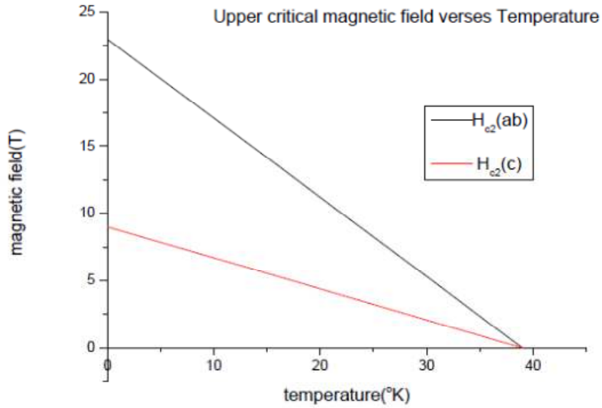
Fig. 1 Upper critical magnetic field versus temperature.
