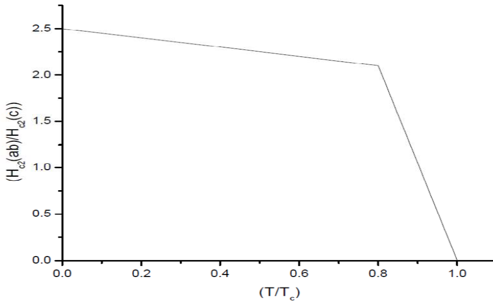
Fig.2 anisotropic property of magnetic field versus temperature.
