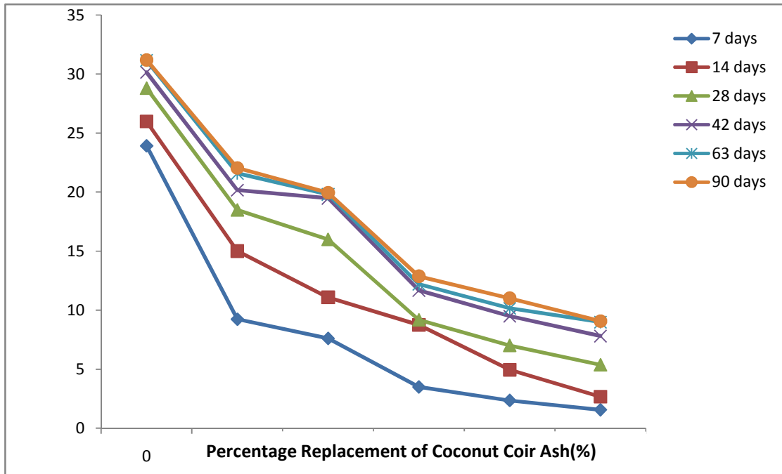
Fig 2: Effect of coconut fibre ash as partial replacement for cement on compressive strenght.
