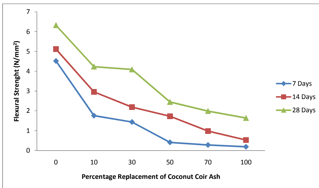
Fig 5: Effect of percentage replacement of coconut fibre ash on flexural strenght (%)
