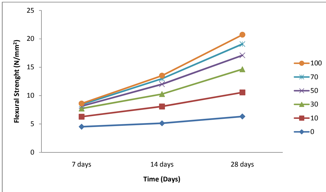
Fig 4: Effect of curing time on flexural strenght
