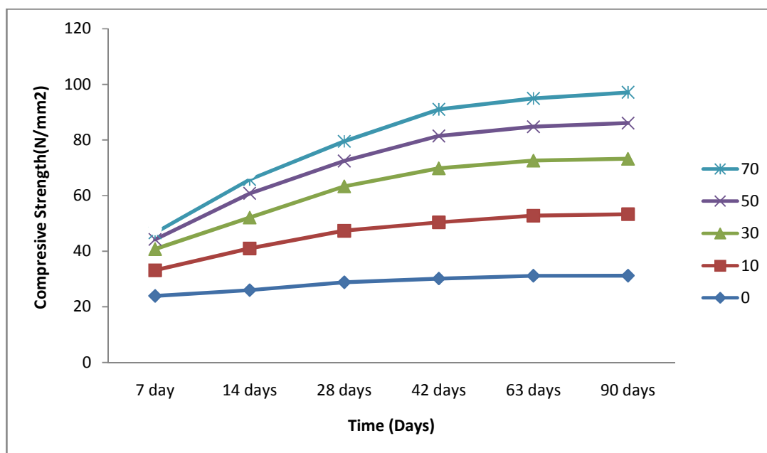
Fig1: Effect of curing time on compressive strength.
