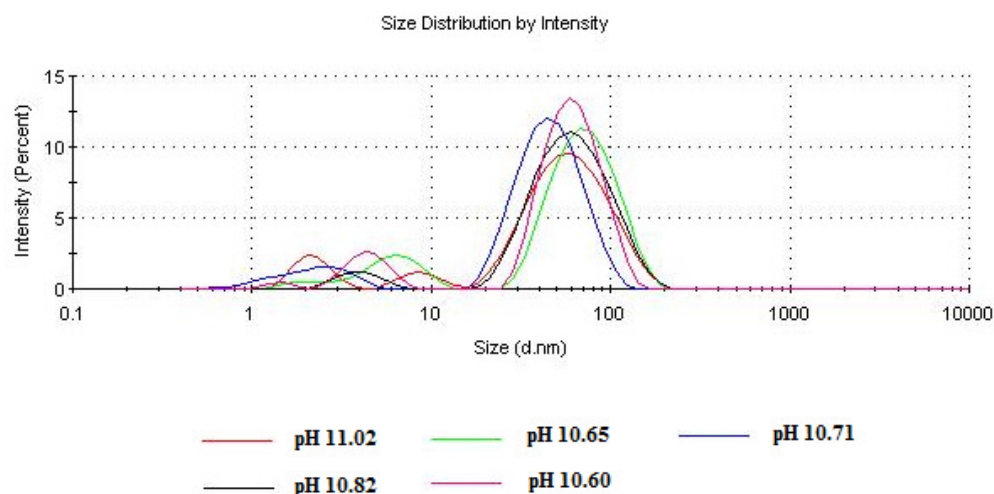
119 Figure 2. Size distribution of silver nanoparticles synthesized at different pH values.
