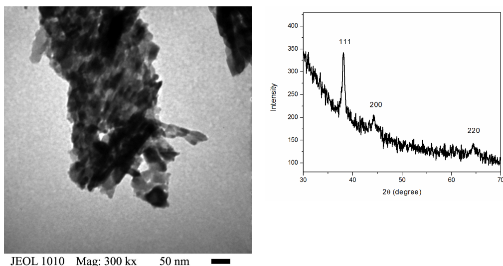
Figure 3. TEM micrograph and powder X-ray diffraction pattern of silver nanoparticles synthesized at pH= 10.65.
