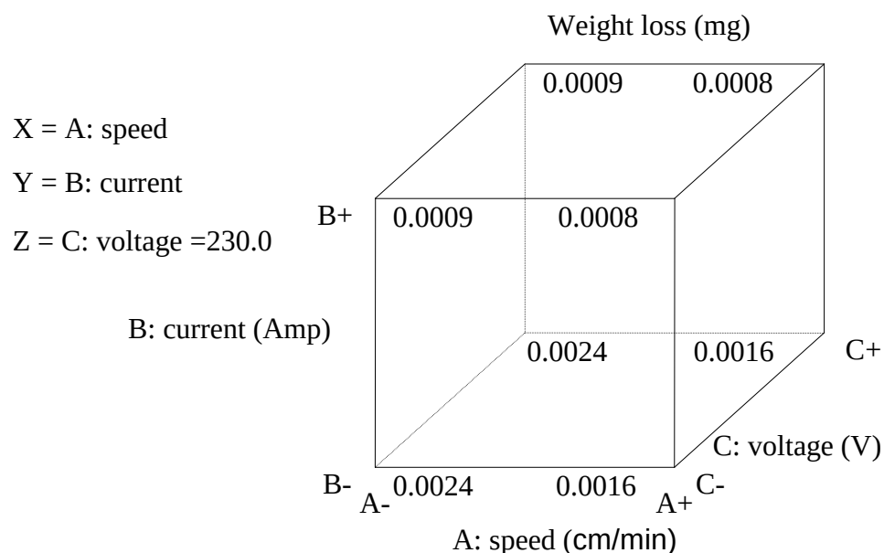
147 Figure 4: Cube plot for ASS in NaOH for 8 days
