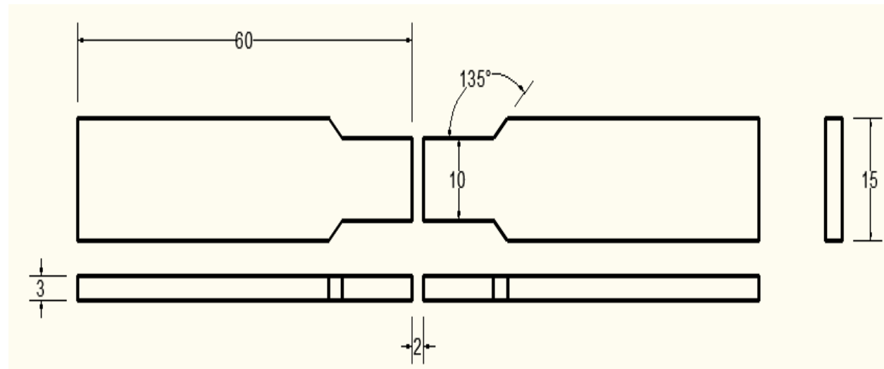
Figure 1: Standard Joint Preparations for plain face sample for welding
