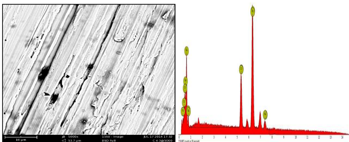
187 Figure 8: Micrograph of FZ C 4 welded and immersed in NaOH for 24 days with EDS profile
