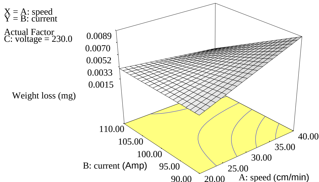
134 Figure 3: Response surface plot for ASS immersed in NaOH for 40 days
