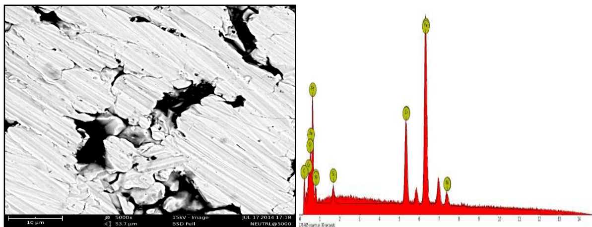
183 Figure 6: Micrograph of the control sample (as received) with EDS profile.
