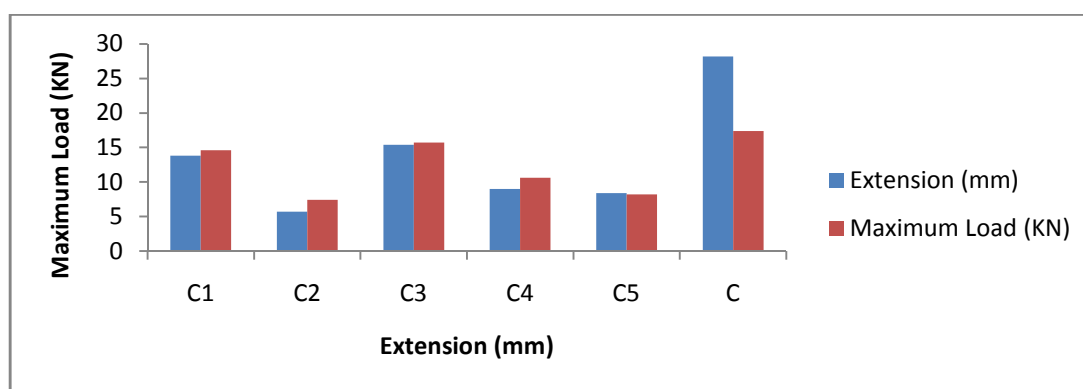
Figure 9: Load-Extension of tensile test on ASS immersed in NaOH medium.
