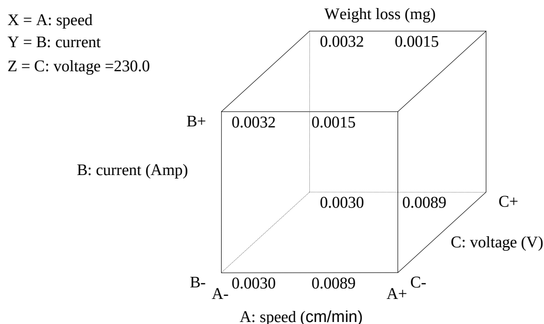
149 Figure 5: Cube plot for ASS immersed in NaOH for 40 days
