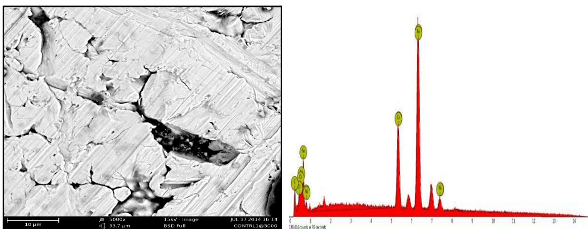
185 Figure 7: Micrograph of the control sample immersed in NaOH for 40 days with EDS profile
