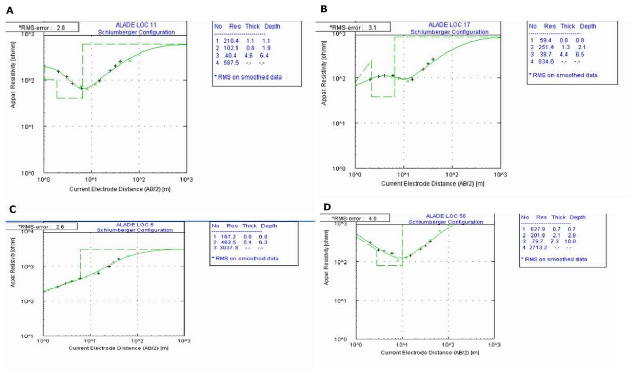
131 Figure 2 : Typical Vertical Electrical Sounding Curves from the Study Area. A : HA curve type, B : KHA curve type, C : A curve type, 132 C : H curve type.
