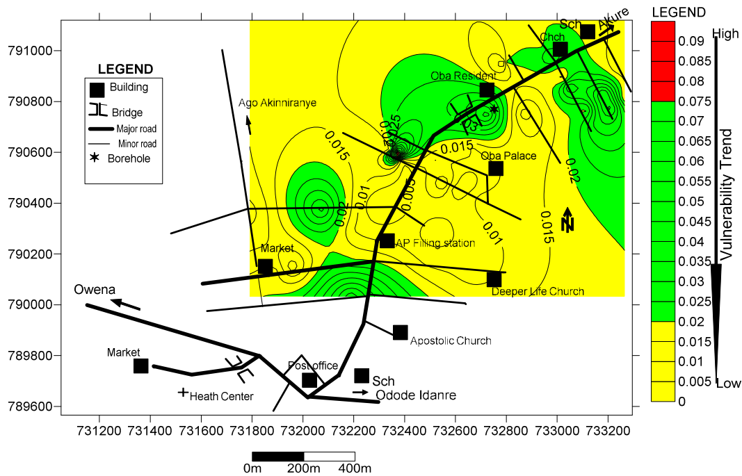
170 Figure 6: Thickness Map showing Longitudinal Conductance from the study area
