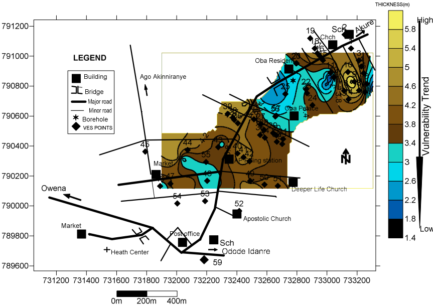
Figure 4: Thickness Map showing unconsolidated materials overlying the basement at Alade.
