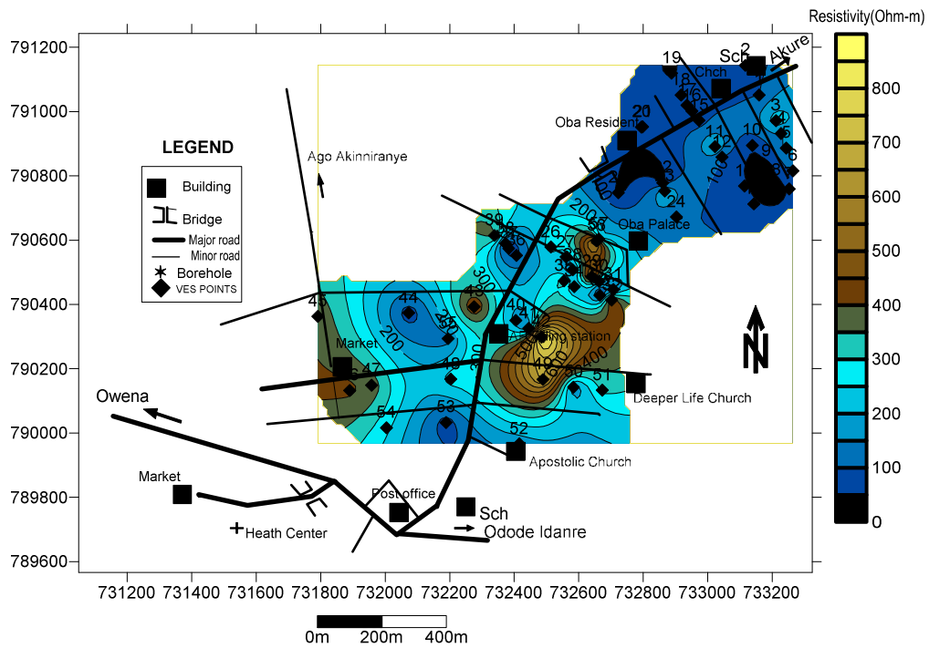
168 Figure 5: Contour Map showing the resistivity distribution of the Aquifer Units
