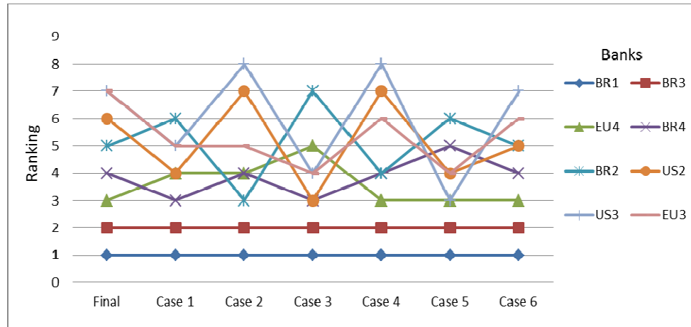
Fig. 5. Ranking variation
