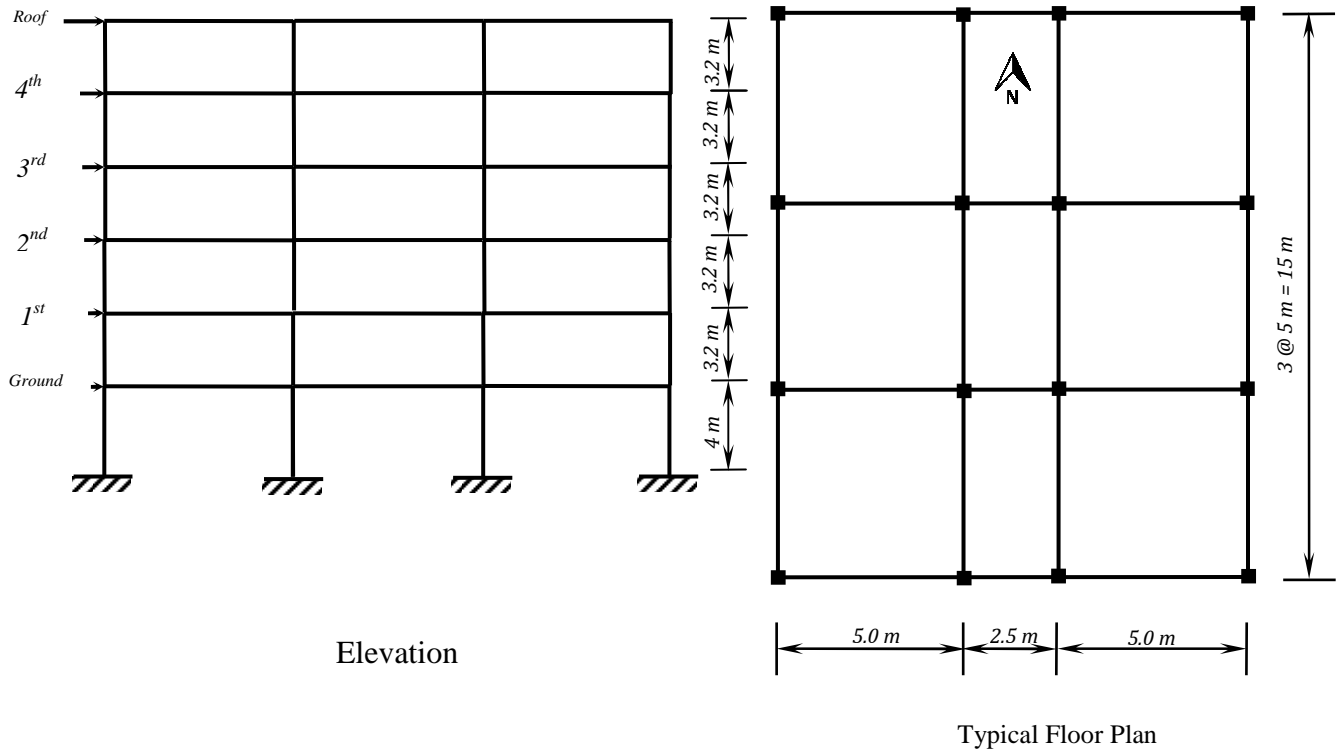
Fig. (1) Dimensions of the Studied Frame Building
