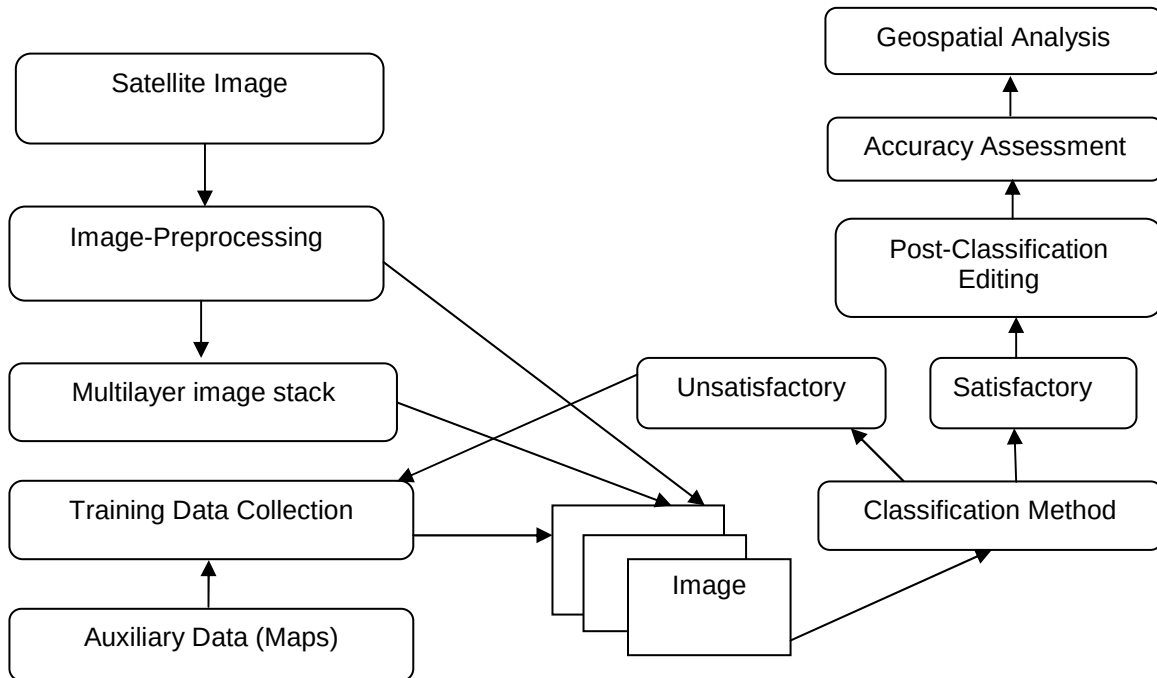
Figure 1: Satellite Image Analysis [Chandra Giri et. al., 2014]
