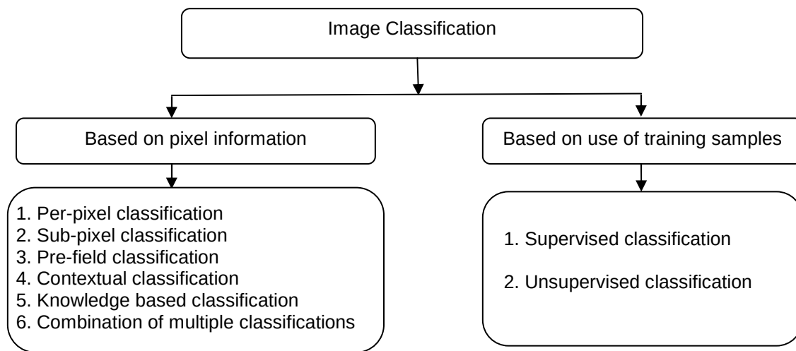
Figure 2: Land Cover Image Classification Approaches [R.Ablin et. al., 2013]
