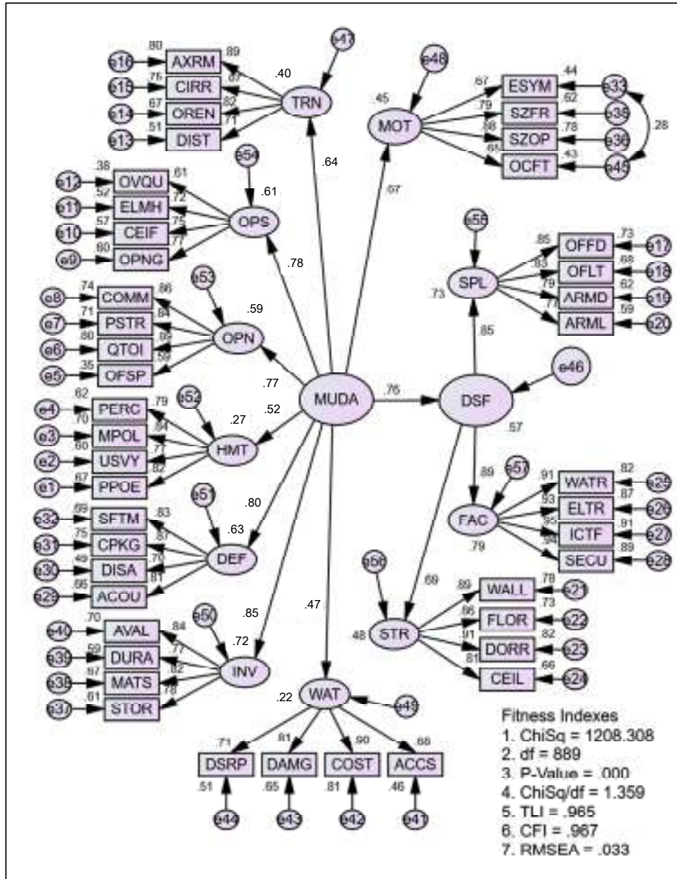
Figure 4. The Proposed Structural Model
