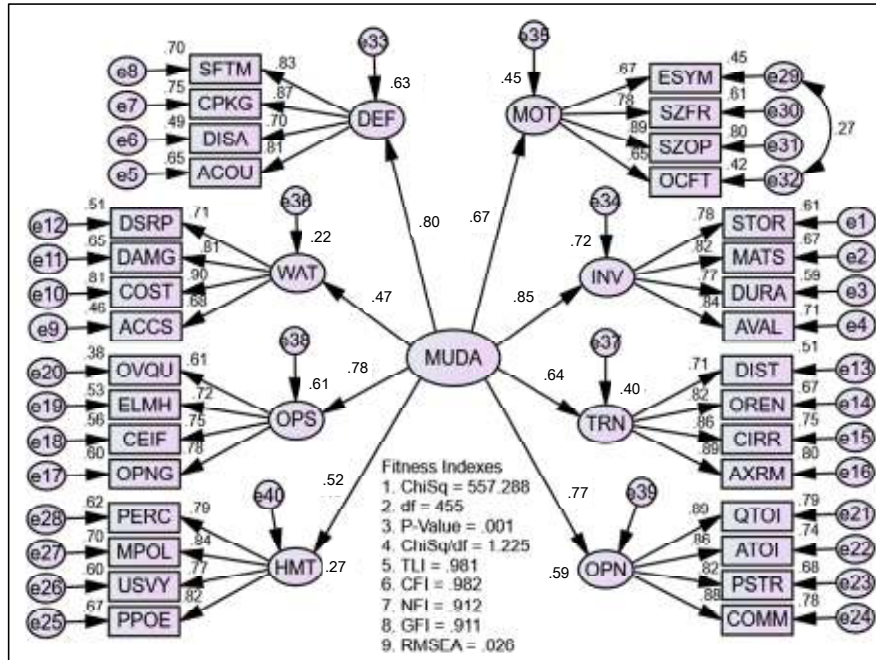
Figure 2. Regression Weights of Sub-constructs Predicting Muda
