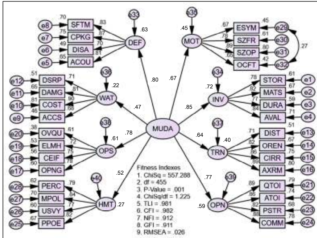
Figure 4: Regression Weights of Sub-constructs Predicting Muda
