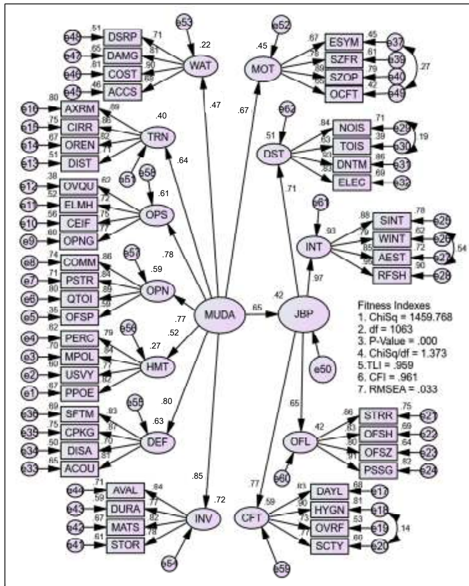
Figure 6: The Proposed Structural Model in Standardized Estimates
