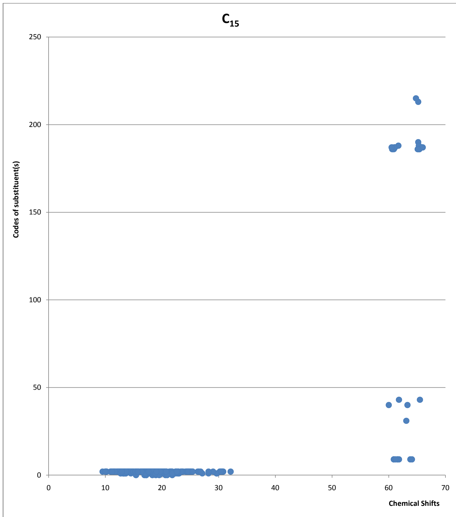
Figure2: Scatter Plots of codes (of substituents) against ^{13}C chemical shifts
