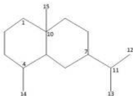
Fig.1: The Eudesmane Skeleton
