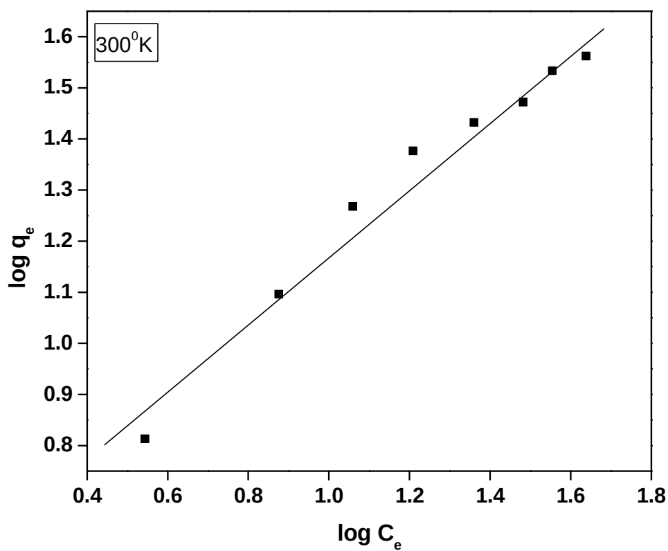
348 349 Fig.-14a: Freundlich plot for adsorption of Congo red by AMSD 350 (adsorption dose 2gm/L. contact time 30 min. and pH 6, 300^0\text{K} ) 351
