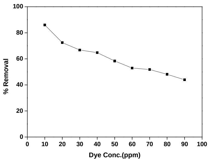
Fig.-12: Effect of Initial dye Concentration on % Removal of Congo red (Initial conc. of Congo red 70 mg/L, adsorption dose 2 gm/L and pH 6.)
