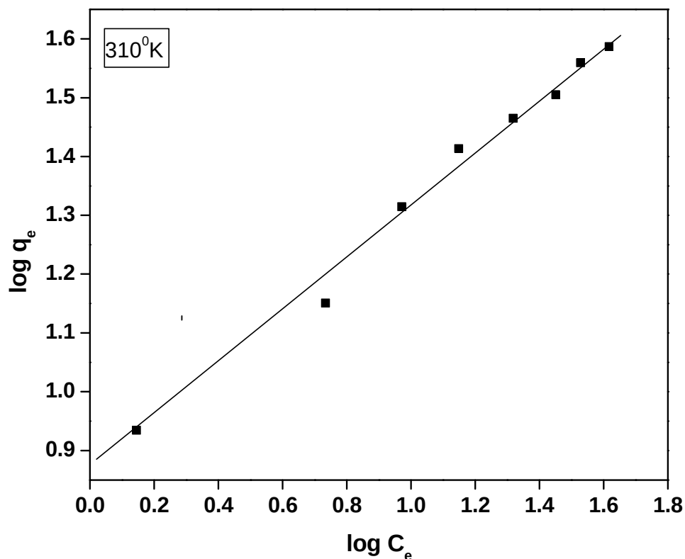
Fig.-14b: Freundlich plot for adsorption of Congo red by AMSD (adsorption dose 2gm/L. contact time 30 min. and pH 6, 310° K)
