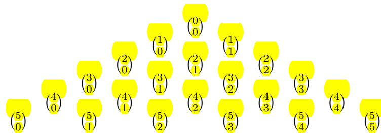
Figure 1: Pascal's Triangle
