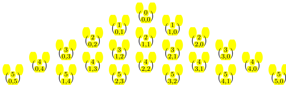
Figure 2: Pascal's Triangle (in multinomial coefficients)
