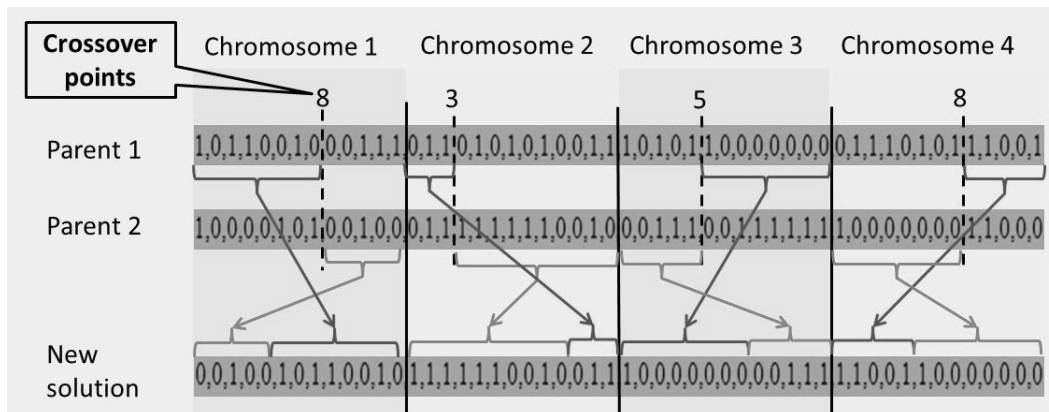
97 Fig. 1. Example of crossover mechanism with 4 chromosomes and 13 genes.
