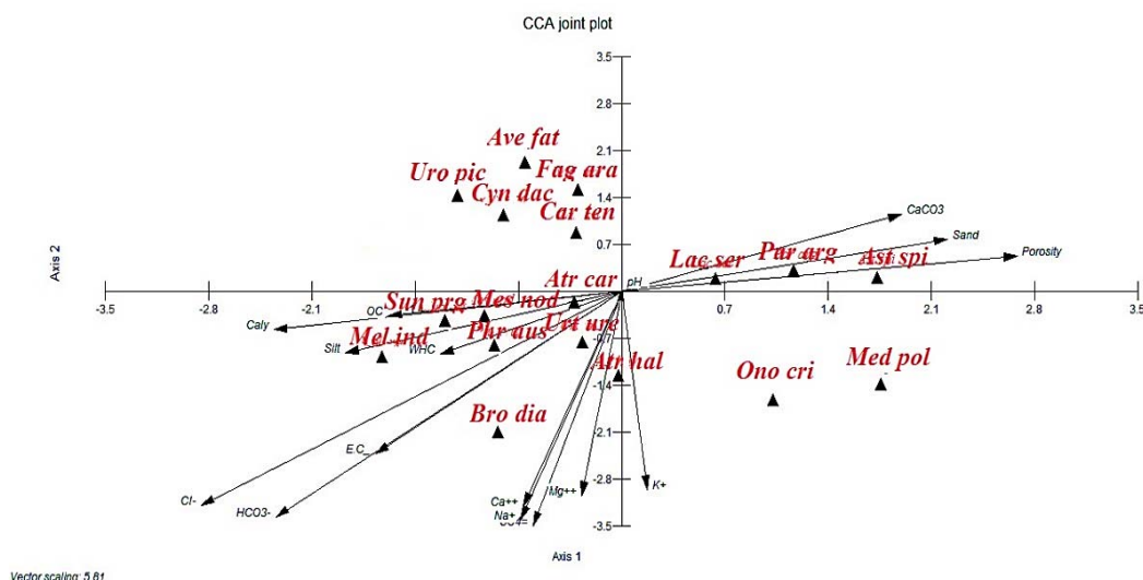
Fig. 4. Canonical Correspondence Analysis (CCA) ordination diagram of the first two axes showing the distribution of the plant species with soil variables in the study area.
