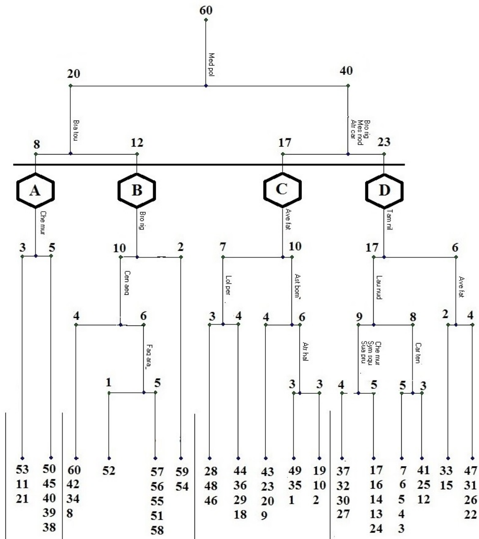
Figure 2. Two Way Indicator Species Analysis (TWINSpan) dendrogram of the 60 sampled stands based on the importance values of the 84 species. The indicator species are abbreviated by the first three letters of genus and species respectively.
