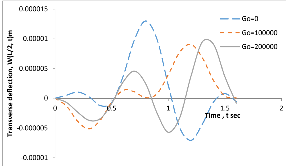
Fig. 5. Displacement profile of a free elastic uniform Bernoulli- Euler beam on constant foundation and traverse by moving distributed for for fixed values of N_o and K_o and various values of G_o .
