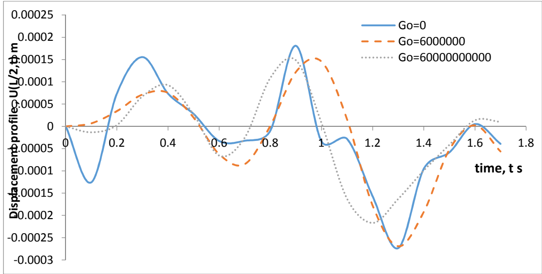
Fig. 2. Displacement profile of a clamped elastic uniform Bernoulli- Euler beam on constant foundation and traverse by moving distributed force for fixed values of No and Ko and various values of Go .
