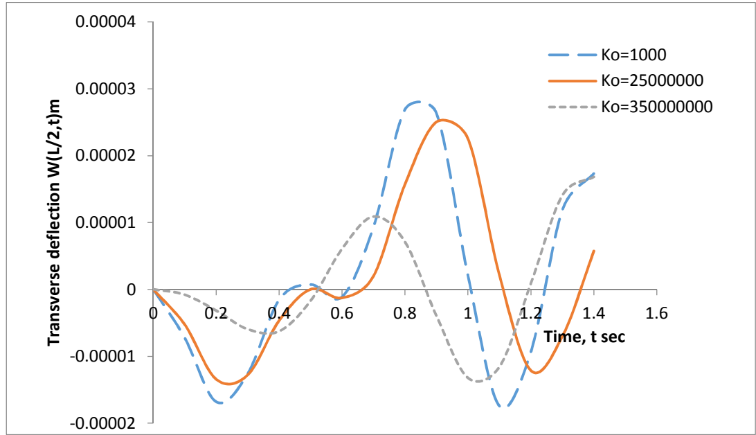
Fig. 4. Displacement profile of a free elastic uniform Bernoulli- Euler beam on constant foundation and traverse by moving distributed for for fixed values of No and Go and various values of Ko .
