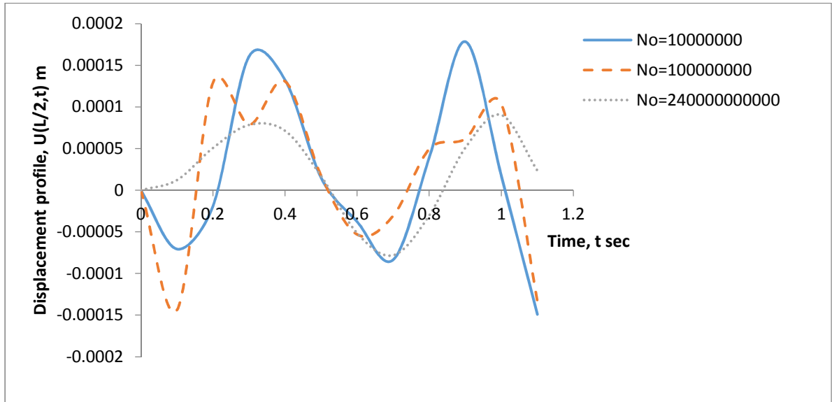
Fig. 3. Displacement profile of a clamped elastic uniform Bernoulli- Euler beam on constant foundation and traverse by moving distributed force for fixed values of Go and Ko and various values of No .
