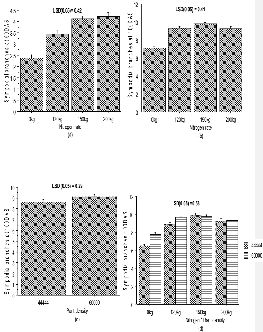
FIG 9: Effects of nitrogen rates at 60 and 100 DAS (a and b), plant density at 100 DAS (c) and interaction of nitrogen with plant density at 100 DAS (d) on sympodial branches
