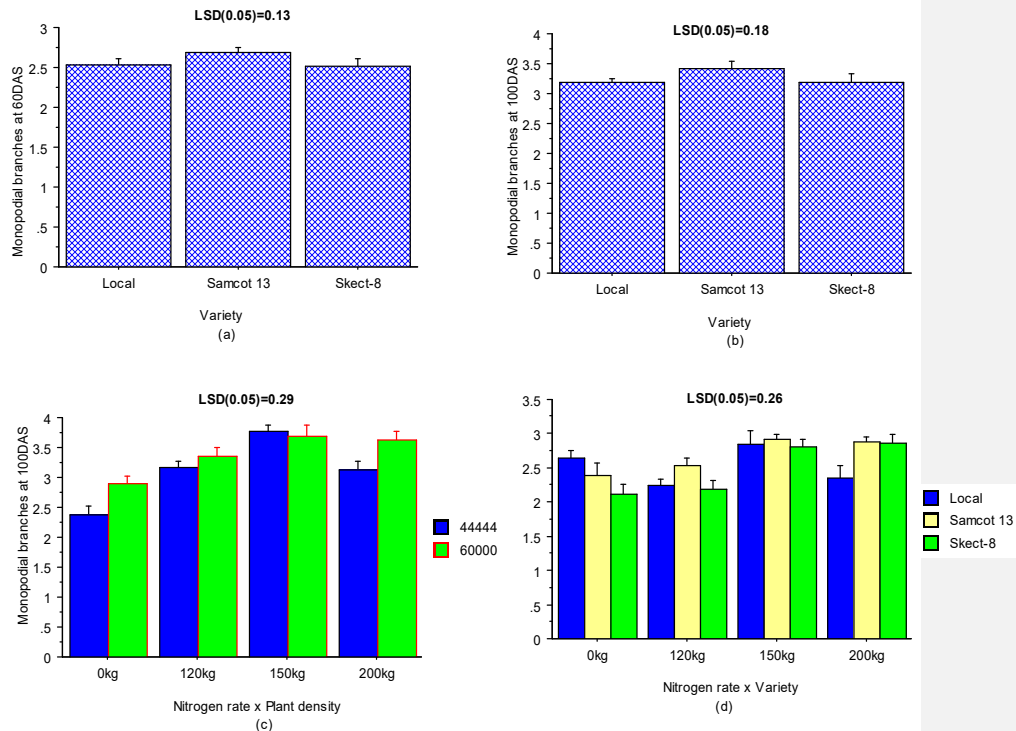
FIG 8: Effects of variety at (a) 60 DAS and (b) 100 DAS and the interaction of N with plant density variety at 100 DAS (c) and nitrogen with variety (d) on monopodial branches of cotton
