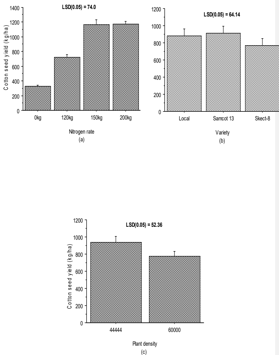
FIG 5: Effects of (a) nitrogen rates, (b) variety and (c) plant density on cottonseed yield (kg/ha)
