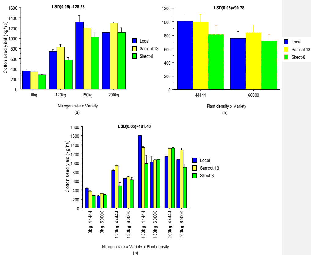
338 FIG 6: Interactive effects of (a) nitrogen x variety, (b) plant density x variety and (c) nitrogen 339 x plant density x variety on cottonseed yield (kg/ha) 340
