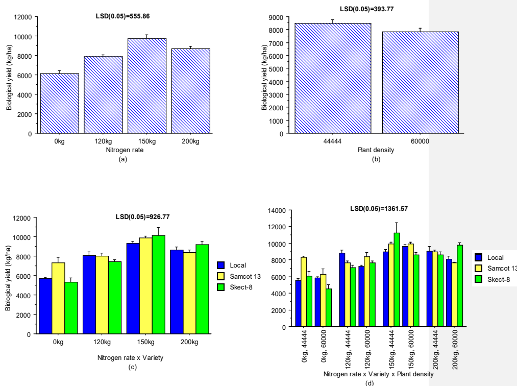
FIG 10: Effect of (a) nitrogen rates, (b) plant density, (c) the interaction of nitrogen with variety and (d) nitrogen with variety with plant density on biological yield
