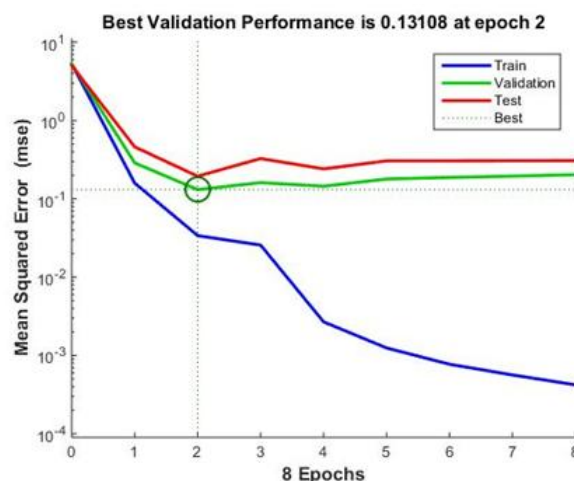
Fig. 2 The BP Training curve
