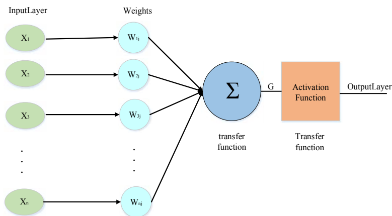
Fig. 3 Structure combining BP and GA
