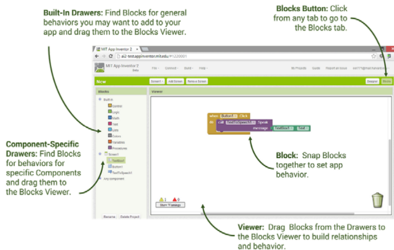
Fig. 10. The Blocks Editor for an app created with App Inventor v. 2.0
