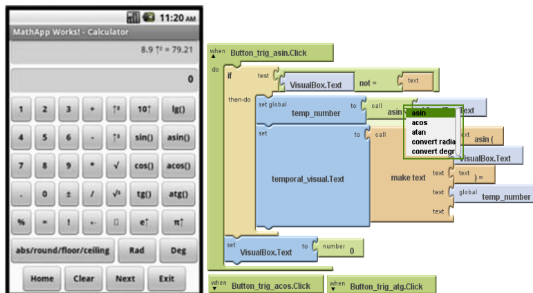
Fig. 14. MathApp Works! Standard version - calculator design view
