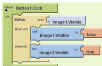
Fig. 7. Visual code vs Textual code for handling the event of a button clicked
