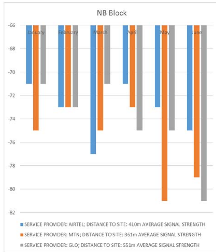
Fig. 6. Graph of signal strength at NB block
