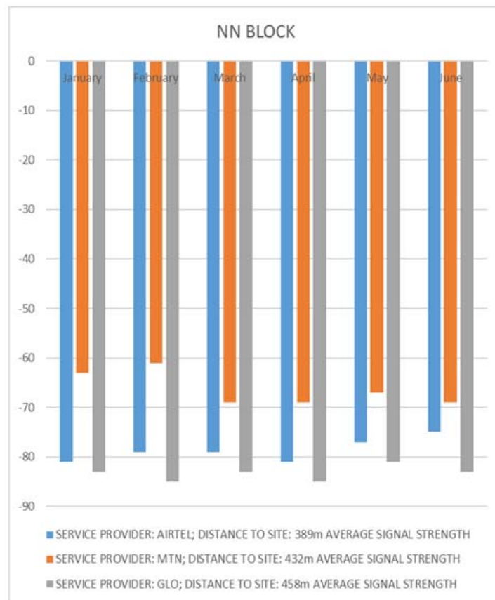
Fig. 4. Graph of signal strength at NN block
