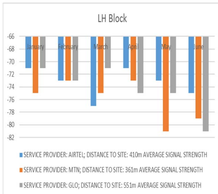
Fig. 5. Graph of signal strength at LH block
