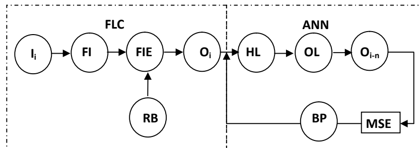
Figure 2 Fuzzy – neuro hybrid control model
