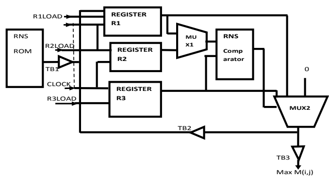
FIG 5.: RNS COMPARATOR SCHEMATIC DIAGRAM
