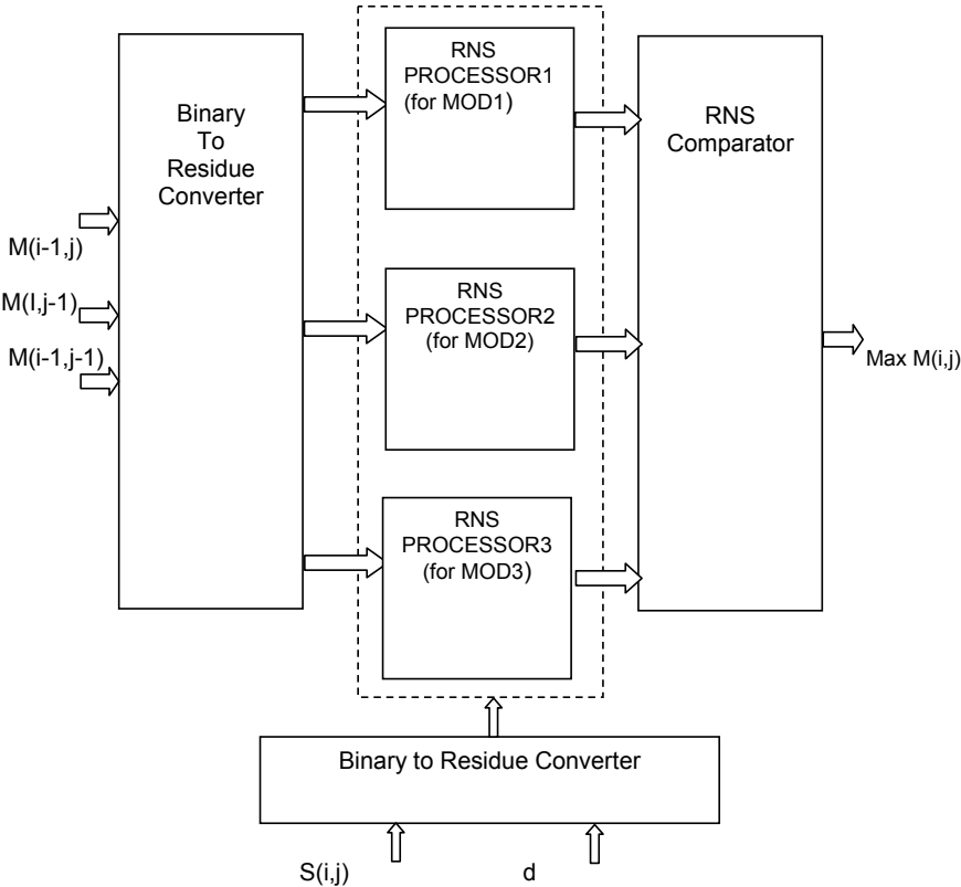
Fig 6: A typical RNS-SWA based signal processor
