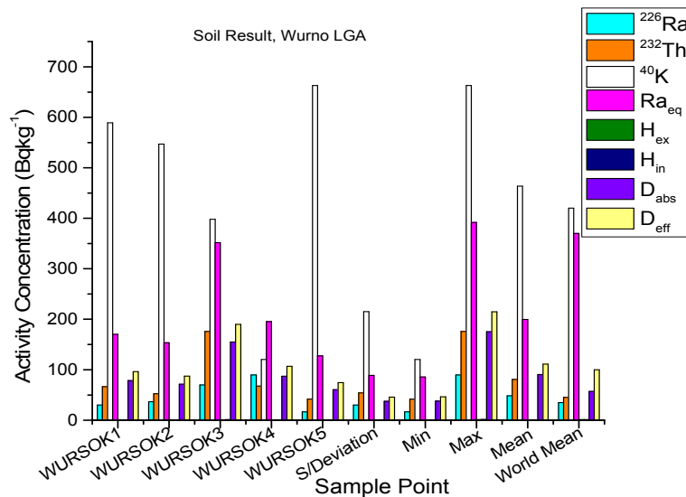
Figure1: A Combined graph of Radionuclides activities and radiological parameters for Soil Samples from Wurno LGA, Sokoto state, Nigeria.
