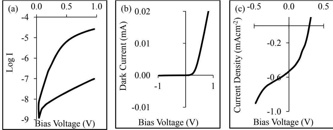
Figure 2. Typical I-V characteristics of the n-CdSe/Au Schottky diodes (a) Log-linear, (b) Linear-linear under dark conditions, and (c) under AM1.5 illumination condition at room temperature.
