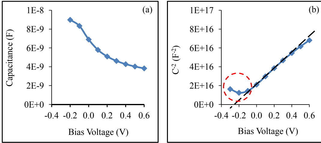
Figure 3. Typical (a) Capacitance vs bias voltage and (b) C^{-2} vs V graphs of the device structure, glass/FTO/n-CdSe/Au. Note: The red dotted circle in Figure 3 (b) signifies the non-linear portion of the Mott-Schottky plot caused by surface states.
