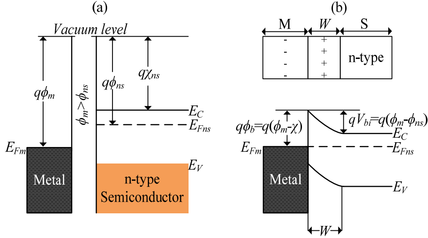
Figure 1. Energy band diagrams illustrating the Schottky contact formation between metal and n-type semiconductor (a) before joining the metal and semiconductor and (b) at equilibrium position after making contact.
