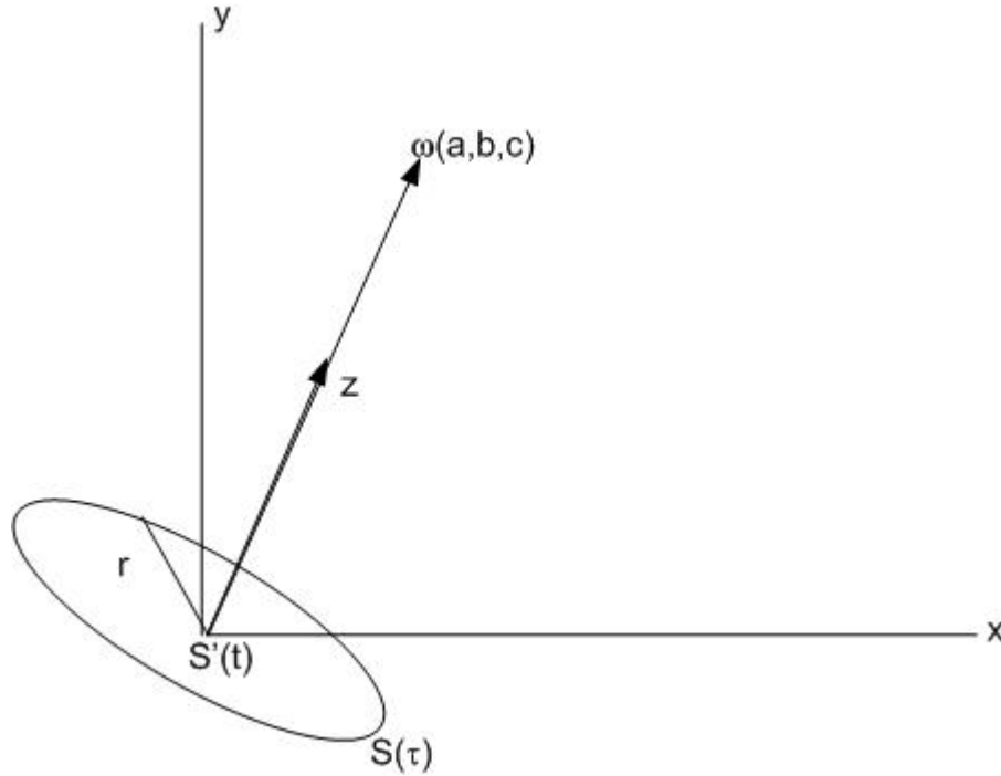
Fig.1. Relationship between rotating and inertial frames
